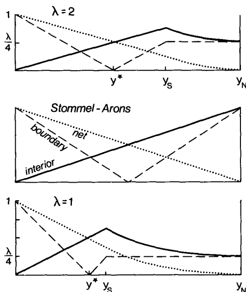
FIG. 5. Interior (solid), boundary (dashed), and net (dotted) transport magnitudes as a function of latitude for \lambda = 2 (upper), \lambda = 1 (lower), and for the Stommel and Arons model (middle). The boundary transport reverses direction at y^* .
