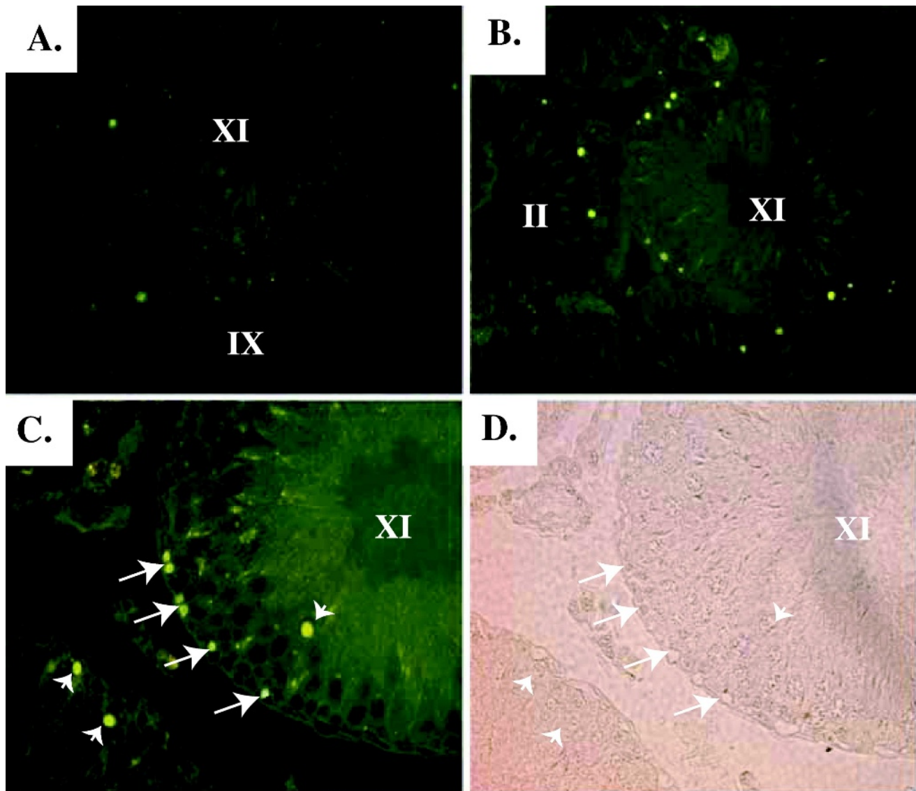
Figure 3. Apoptosis (TUNEL) analyses in the testes P60 F2 generation SD rats from control (A) and vinclozolin (B) at 200 \times magnification and vinclozolin (C) and phase contrast (D) at 400 \times magnification. Apoptotic TUNEL positive cells labeled yellow. Arrows indicate possible spermatogonial cells along the basement membrane. Arrowheads indicate spermatocytes within the seminiferous tubule, and the lumen is depicted with a roman numeral indicating the approximate stage of the cycle of seminiferous epithelium. Micrographs are representative of a minimum of 10 different analyses of F2 vinclozolin generation animals.
