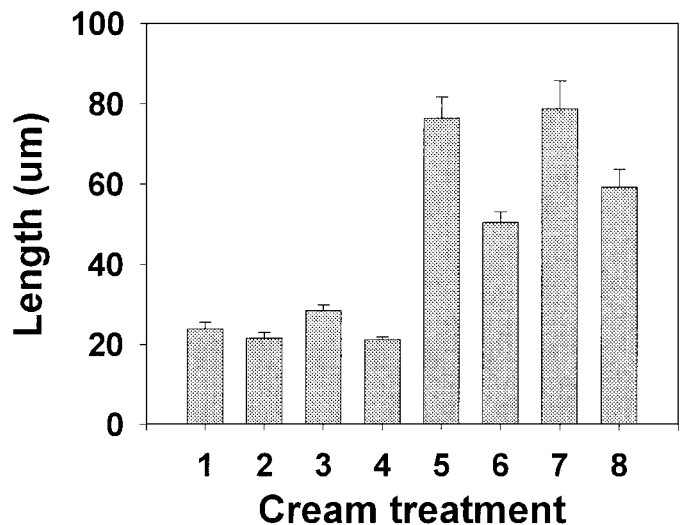
Figure 5. Lamella lengths in fresh (bars 1 to 4) and aged (bars 5 to 8) foams prepared from four cream treatments. Results are the average of thirty images per treatment; error bars represent standard error. 1 = HTST pasteurized, unstabilized, fresh foam; 2 = HTST pasteurized, stabilized, fresh foam; 3 = UHT sterilized, unstabilized, fresh foam; 4 = UHT sterilized, stabilized, fresh foam; 5 = HTST pasteurized, unstabilized, foam aged 24 h; 6 = HTST pasteurized, stabilized foam aged 24 h; 7 = UHT sterilized, unstabilized foam aged 24 h; and 8 = UHT sterilized, stabilized foam aged 24 h.
