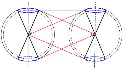
FIG. 2: Precessional coupling by stereographic projection: mutual geometric interaction of oscillators.
