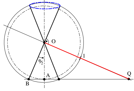
FIG. 1: Oscillation by precession on the sphere S^2 with amplitude r = 2|A - B| (blue) stereographically projected to the Coulomb distance r_c = |O - Q| (red) with r = 2 \sin(\theta/2) and r_c = \cot(\theta/2) . The horizontal distance d = |A - Q| = |A - O|^2/|A - B| = \cos(\theta/2)r_c = (1 + \cos \theta)/r .
