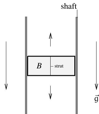
Figure 1: Sliding box filled with radiation in a gravitational field \vec{g} .
