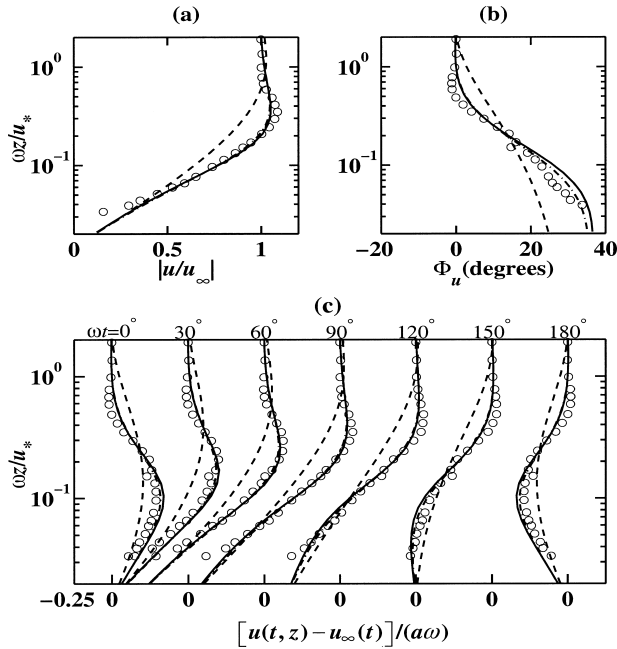
FIG. 2. The predicted and measured (a) magnitude and (b) phase of the dimensionless complex amplitude of velocity, u/u_* , for the wave boundary layer over a rough bed. (c) Evolution of dimensionless velocity defect, [u(t, z) - u_\infty(t)]/a\omega over one-half wave cycle for a free-stream velocity of u_\infty = a\omega \sin\omega t : analytical solution (2.34) (solid lines) and numerical solution (dashed-dot lines) of viscoelastic-diffusion model; the eddy viscosity model solution (2.32b) (dashed lines); Van Doorn (1982) observations (circles).
