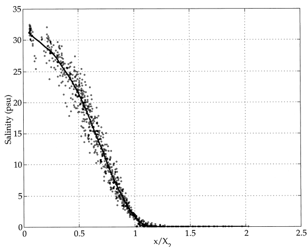
FIG. 5. Depth-averaged salinity as a function of x/X_2 ; X_2 was determined directly from bottom salinity measurements; data taken from USGS CTD transects 1988–92.
