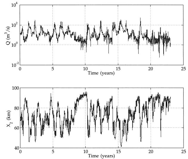
FIG. 3. Daily time series of river flow and salinity intrusion length scale X_2 . The data series starts on 1 Oct 1967.
