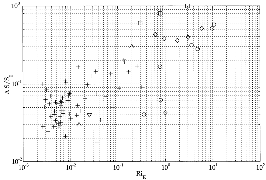
FIG. 14. Effect of Ri_E on estuarine stratification. Data taken from USGS CTD transects are the average along transect of top - bottom salinity difference for USGS from (+) 1988-93, (○) 1996-97, and (◇) 1998-99. Other data are taken from Fischer (1972) and represent the Vellar (□), the Gironde (△), and the Mersey (▽) estuaries.
