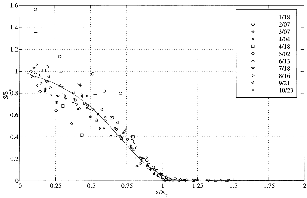
FIG. 8. Salinity distributions from water year 1995. Dates corresponding to symbols are shown on plot. The solid line is the dimensionless function derived from the spline fit to the 1988–93 data with the salinity at x = 0 scaled by the corresponding salinity at the Golden Gate.
