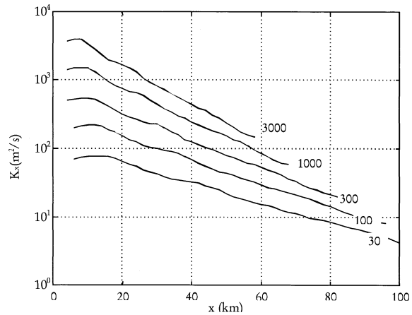
FIG. 10. Plot of K_x (\text{m}^2 \text{ s}^{-1}) as a function of position in the estuary for five different flow rates ( \text{m}^3 \text{ s}^{-1} ).
