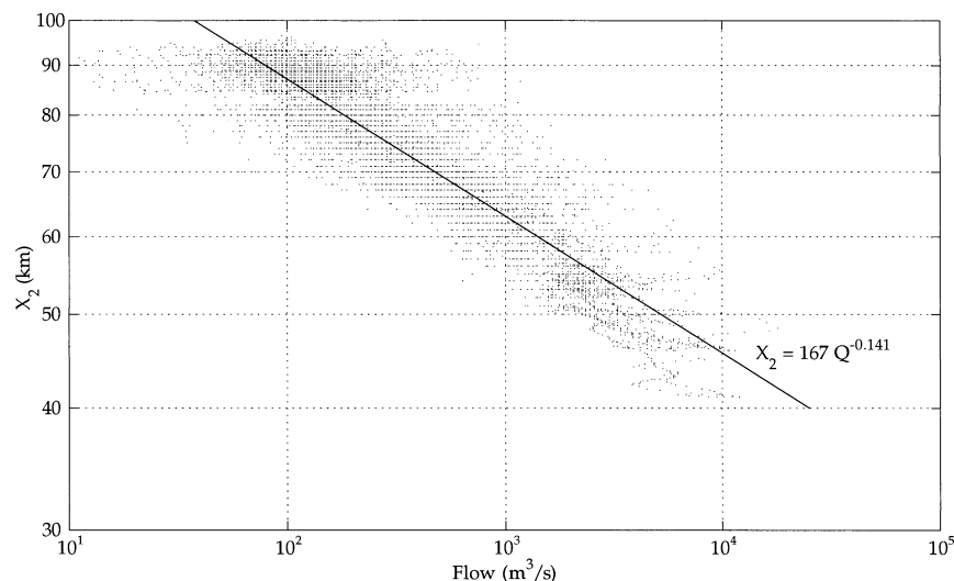
FIG. 4. Functional relationship between river flow, Q , and X_2 . The line shown is the steady-state best-fit Q - X_2 relation given by Eq. (10).
