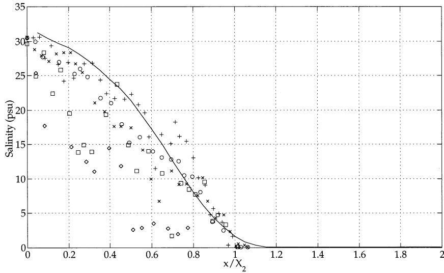
FIG. 6. An example of non-self-similar salinity distributions from Feb–Apr 1986 (data from USGS/USBR). Symbols represent: ( \diamond ) 25 Feb, Q = 7900 \text{ m}^3 \text{ s}^{-1} ; ( \square ) 20 Mar, Q = 4700 \text{ m}^3 \text{ s}^{-1} ; ( \circ ) 25 Mar, Q = 3200 \text{ m}^3 \text{ s}^{-1} ; ( \times ) 8 Apr, Q = 1900 \text{ m}^3 \text{ s}^{-1} ; ( + ) 18 Apr, Q = 1200 \text{ m}^3 \text{ s}^{-1} .
