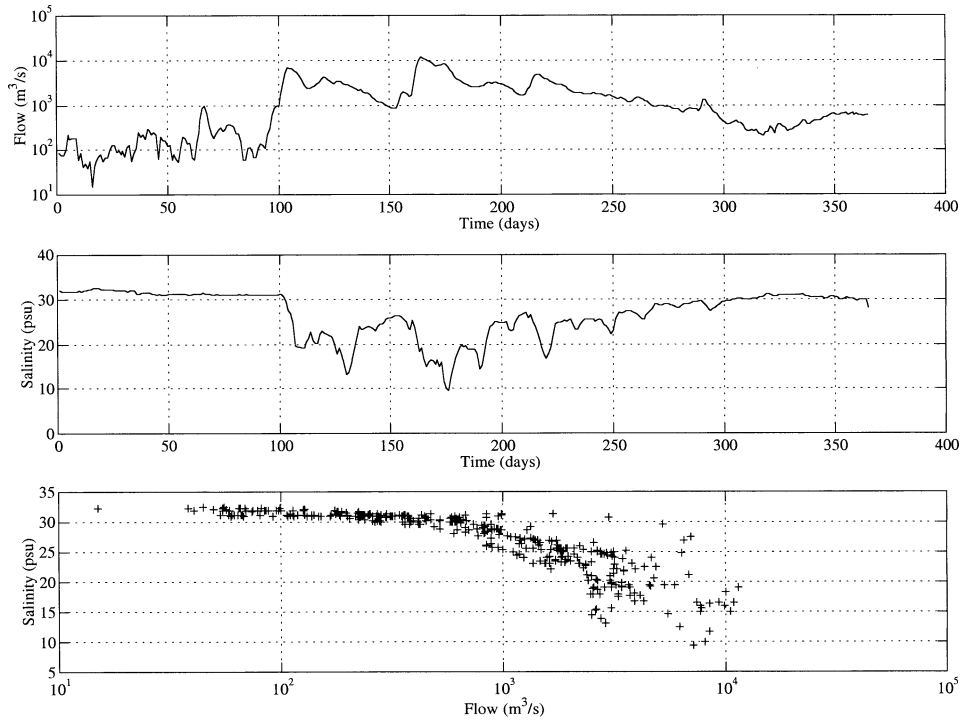
FIG. 7. Flows and salinity at the Golden Gate for water year 1995.
