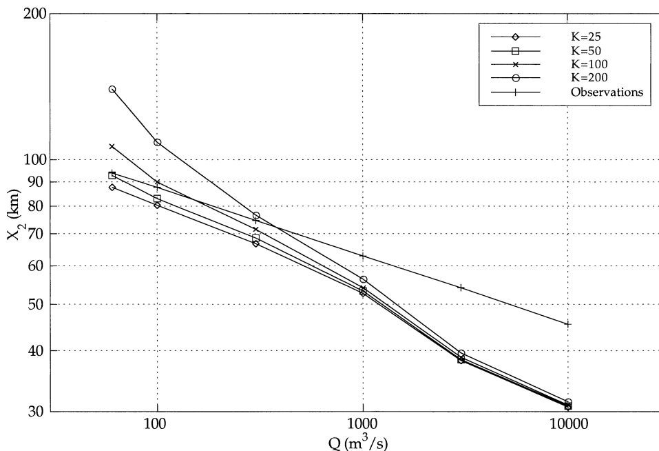
FIG. 12. Steady-state X_2 - Q relations computed numerically using different values of K_b and keeping \gamma constant compared with observed values.
