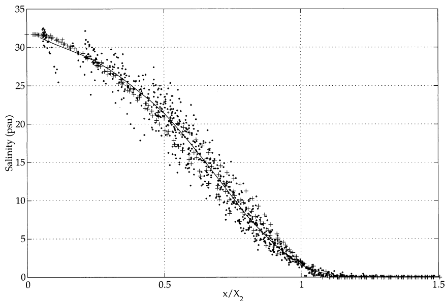
FIG. 13. Computed salinity distributions as functions of distance from the Golden Gate normalized by X_2(Q) for K_B = 30 \text{ m}^2 \text{ s}^{-1} and with \gamma varying between 0.081 and 0.054 depending on flow. The (+) represent computed salinities for flows between 100 and 10 000 \text{m}^3 \text{s}^{-1} , the (o) represent USGS observations, and the solid line is the spline fit to the USGS data.
