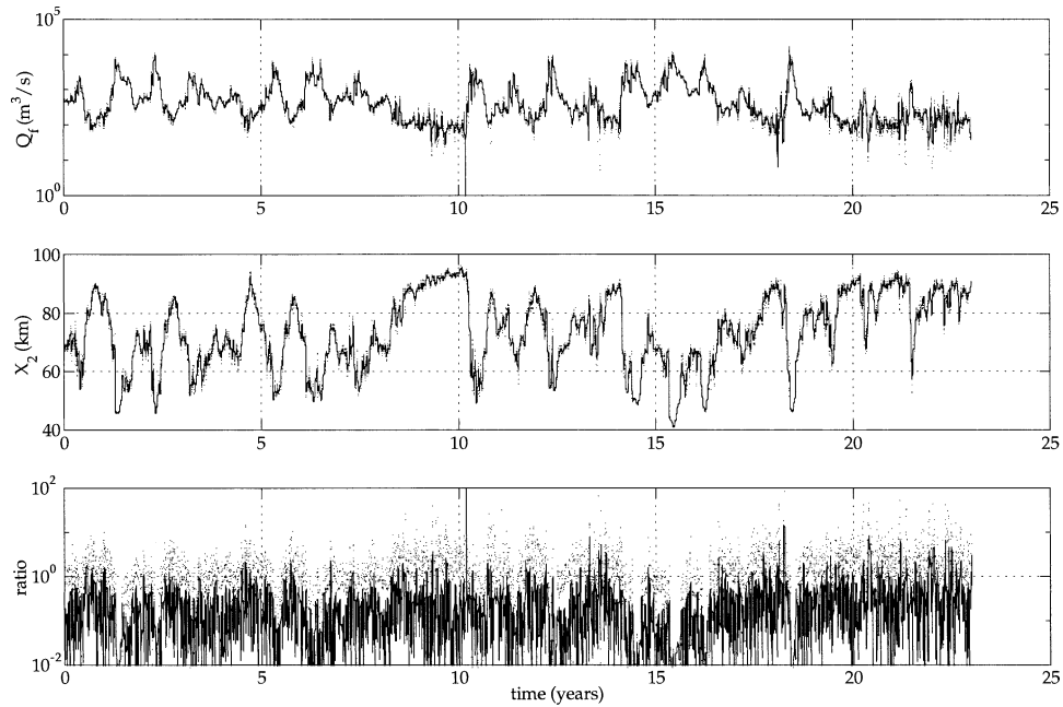
FIG. A1. Plot of (a) Q_f ( \text{m}^3 \text{s}^{-1} ), (b) X_2 (km), and (c) ratio of \partial S/\partial t: u\partial S/\partial x . The dots represent the raw daily data and the lines represent the raw data low-pass filtered with a fourth-order Butterworth filter with a 14-day time constant.
