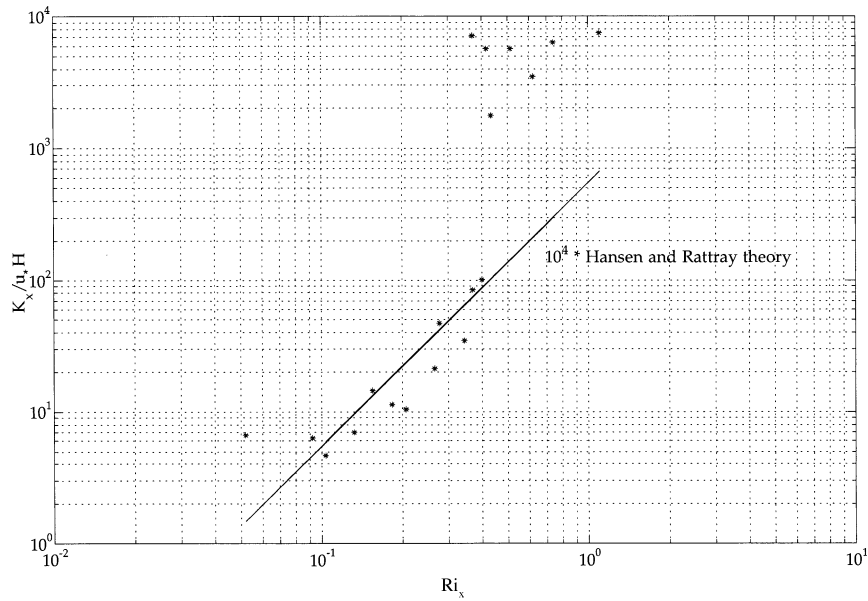
FIG. 16. The dependence of K_x/(u_*H) on Ri_x , as computed using a one-dimensional water column model that includes tidally varying stratification.
