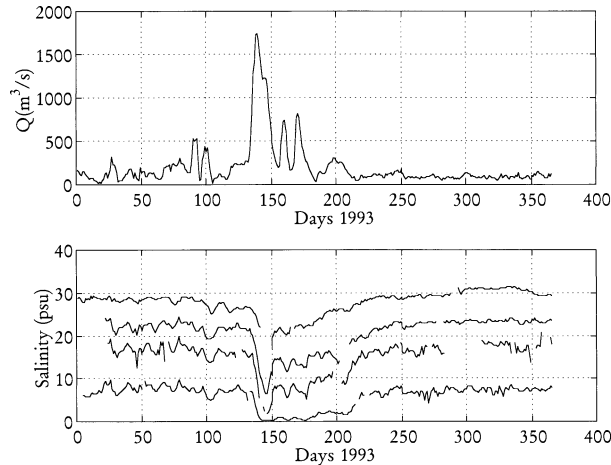
FIG. 2. Flow and salinity variability in 1993 in northern San Francisco Bay. The four salinity stations shown are located at x = 19.4, 40.5, 50.5, and 72.5 km.
