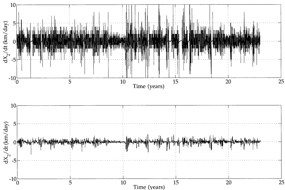
FIG A2. Time series of (a) raw dX_2/dt and (b) low-pass filtered dX_2/dt .
