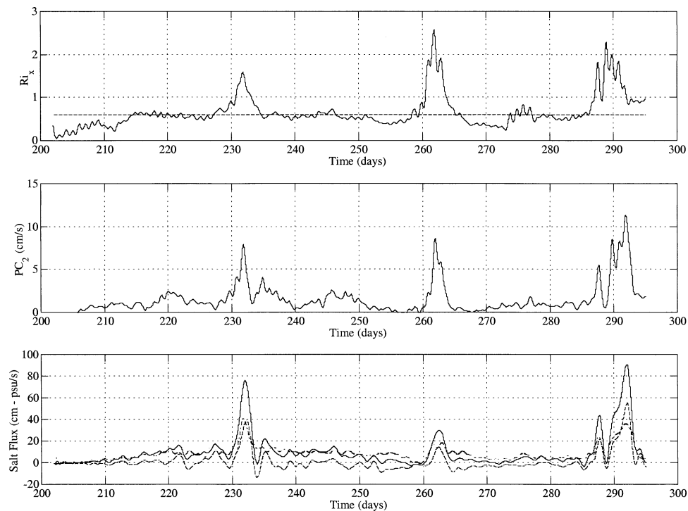
FIG. 15. Salt flux and stability in Susiun Cut 1995: (a) Ri_x (solid line) computed from observed tidal currents and dS/dx —the critical value of Ri_x = 0.6 is also shown (dashed line); (b) strength of gravitational circulation PC_2 ( \text{cm s}^{-1} ); (c) near-bottom salt flux (+ upstream), decomposed as total salt flux (solid line), salt flux due to tidal averages \langle U \rangle \langle S \rangle (dot-dash line), and salt flux due to tidally fluctuating salinities and velocity \langle U'S' \rangle (dashed line), where U' and S' are the instantaneous deviations from the low-pass filtered values \langle U \rangle and \langle S \rangle .
