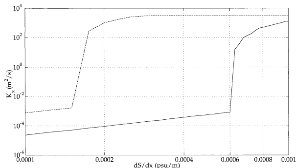
FIG. 17. Plot of K_x as a function of dS/dx averaged over two spring–neap cycles: solid line is 10 m and dashed line is 20 m. The instantaneous values of K_x used are those given in Fig. 16.
