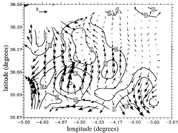
FIG. 5. Horizontal distribution at z = -253 m of the vertical shear \mathbf{u}_z for survey 1. Reference vector is 2 \times 10^{-3} \text{ s}^{-1} . Only every other vector has been plotted. Isolines indicate the magnitude |\mathbf{u}_z| with \Delta = 1 \times 10^{-3} \text{ s}^{-1} .
