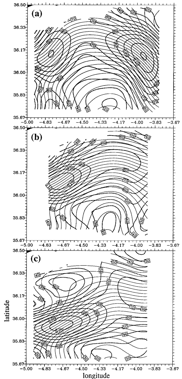
FIG. 7. Horizontal distribution of the geostrophic speed (dotted thick isolines with \Delta = 10 \text{ cm s}^{-1} ) and pressure anomaly [ \Psi(\mathbf{x}, z_1, z) ] isolines (continuous thin lines) at z = -13 m using a reference level z_1 = -253 m, for (a) survey 1, (b) survey 2, and (c) survey 3. The pressure anomaly field has been plotted just to indicate the direction of the geostrophic flow (tangent to the pressure anomaly isolines).
