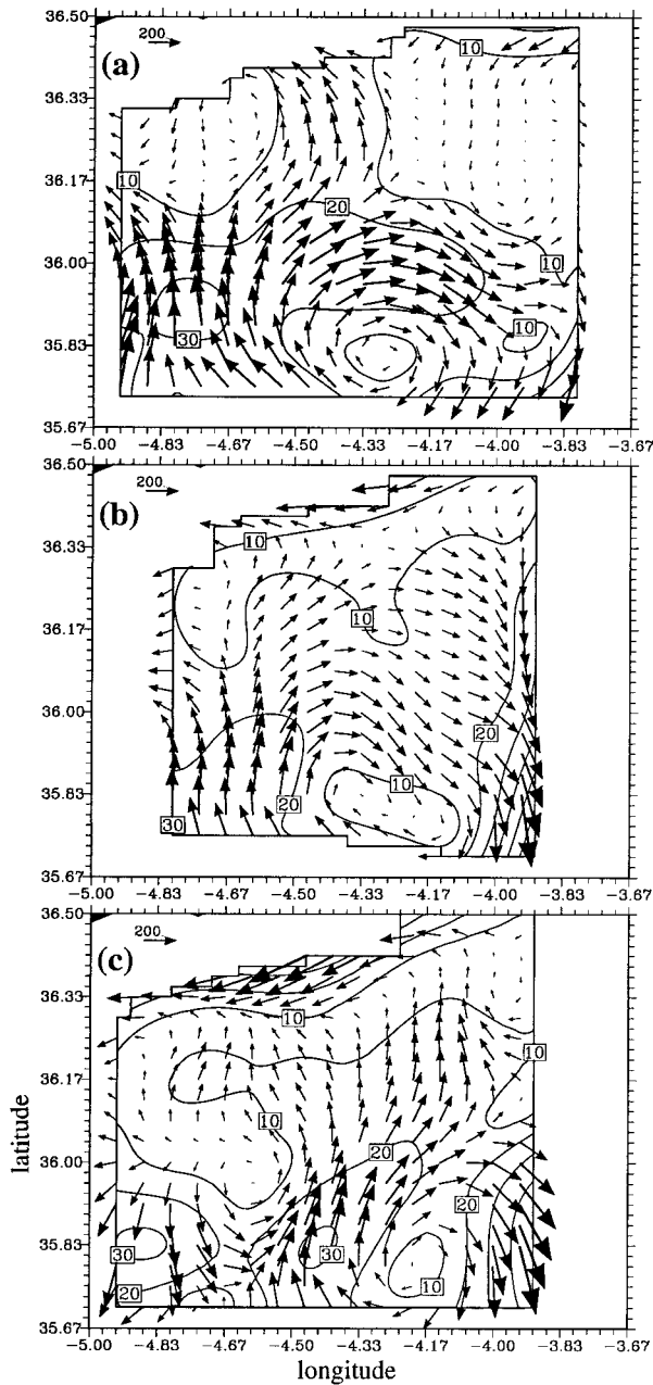
FIG. 9. Horizontal distribution at z = -100 m of the ageostrophic velocity field \mathbf{u} - \mathbf{u}^g for (a) survey 1, (b) survey 2, and (c) survey 3. Reference vector is 20 \text{ cm s}^{-1} . Only every other vector has been plotted. Isolines indicate the vector magnitude with \Delta = 10 \text{ cm s}^{-1} . The geostrophic velocity at the reference level has been neglected.
