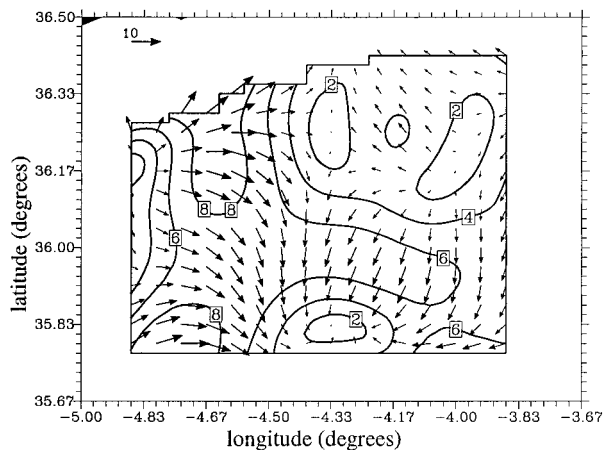
FIG. 17. Horizontal distribution of the gradient imbalance \mathbf{I}_1(\mathbf{x}, z_1) at the reference level z_1 = -253 m in survey 1. Reference vector is 10 \times 10^{-6} \text{ m s}^{-2} . Only every other vector has been plotted. Isolines indicate the magnitude |\mathbf{I}_1(\mathbf{x}, z_1)| with \Delta = 1 \times 10^{-6} \text{ m s}^{-2} .
