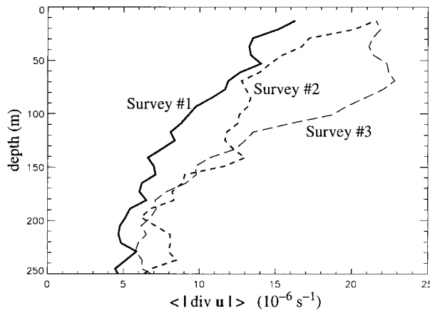
FIG. A2. The horizontal average of the absolute value of the horizontal divergence \langle |\nabla \cdot \mathbf{u}| \rangle as a function of depth for the three surveys.
