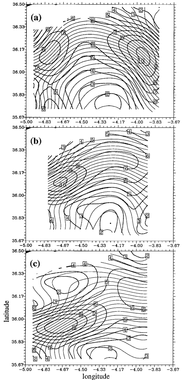
FIG. 10. Horizontal distribution at z = -13 m of the magnitude of the pressure anomaly gradient force -\nabla \Psi(\mathbf{x}, z_1, z) for z_1 = -253 m (dotted thick isolines with \Delta = 1 \times 10^{-5} \text{ m s}^{-2} ). The pressure anomaly field ( \Psi , thin continuous isolines) has been plotted just to indicate the direction of the pressure anomaly force (normal to the pressure anomaly isolines with a northward component).
