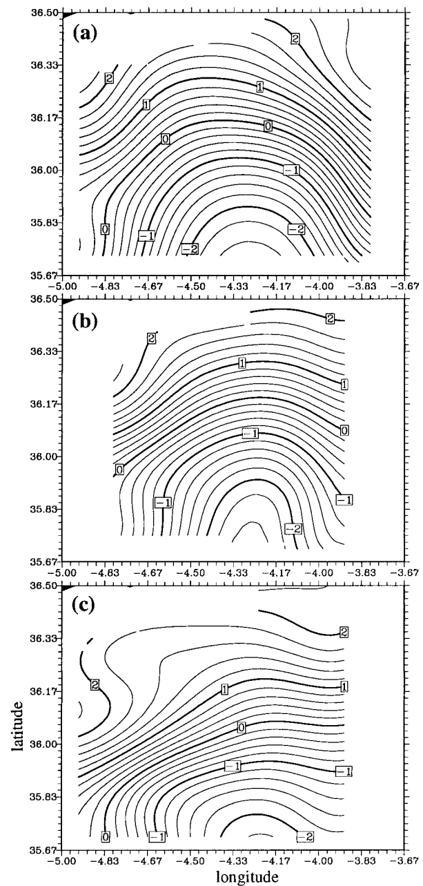
FIG. 6. Horizontal distribution of the geostrophic transport function Q_{z_1}(\mathbf{x}, z) , at depth z = -13 m and for the reference level z_1 = -253 m, for (a) survey 1, (b) survey 2, and (c) survey 3; \Delta = 0.2 \times 10^6 \text{ m}^3 \text{ s}^{-1} .
