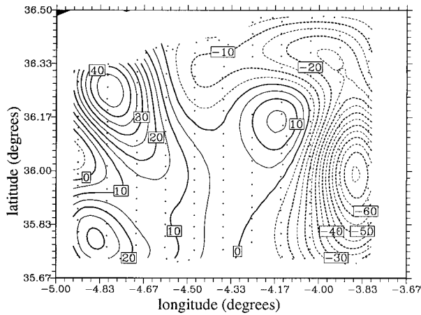
FIG. 13. Horizontal distribution at z = -100 m of the QG vertical velocity w^{\text{QG}} for survey 1; \Delta = 5 \times 10^{-5} \text{ m s}^{-1} .
