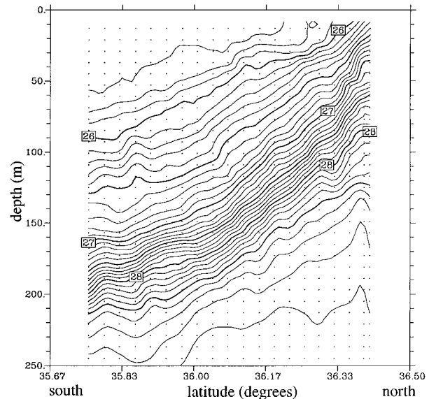
FIG. 2. Potential density ( \sigma_\theta ) distribution at vertical section F for survey 1 (referenced in Fig. 1). The dots indicate the interpolated SeaSoar data. Contour interval \Delta = 0.1 \sigma_\theta .
