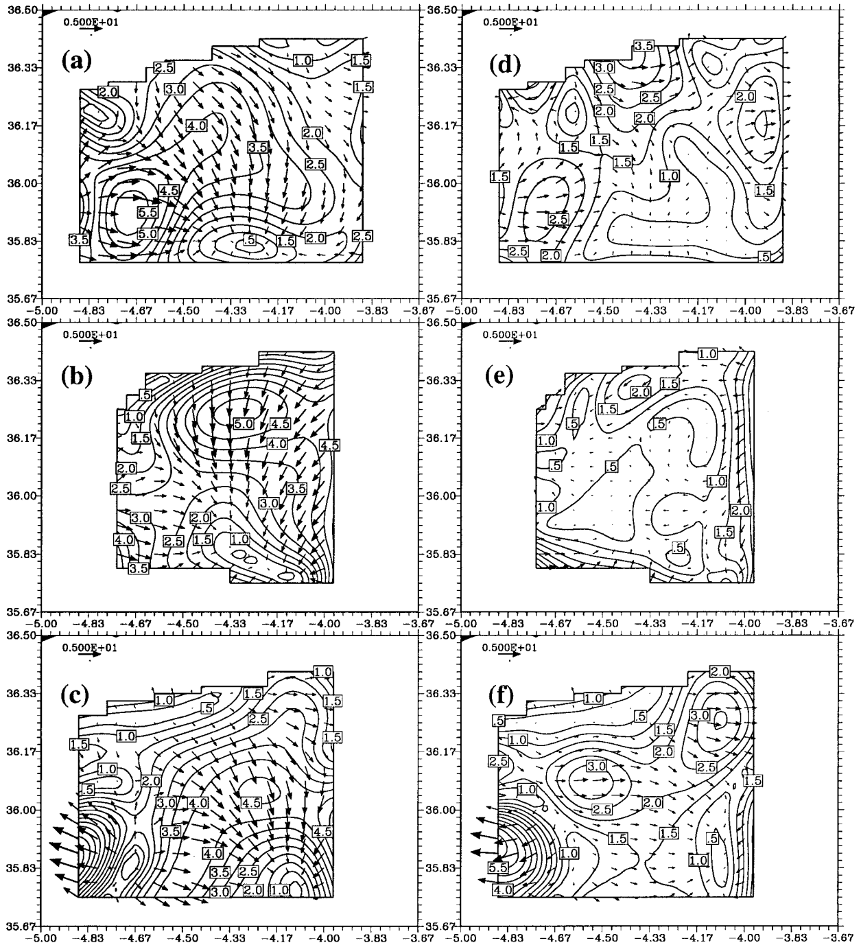
FIG. 16. Horizontal distribution at z = -13 m of the geostrophic imbalance I_0(x, z_1, z) (a, b, and c), and the gradient imbalance I_1(x, z_1, z) (d, e, and f), with z_1 = -253 m, for the three surveys 1, 2, and 3, respectively. Reference vector is 5 \times 10^{-5} \text{ m s}^{-2} . Vectors close to the boundary stations have been removed because of the impossibility of obtaining realistic spatial derivatives there. Only every other vector has been plotted. Isolines indicate the vector magnitude with \Delta = 0.5 \times 10^{-5} \text{ m s}^{-2} .
