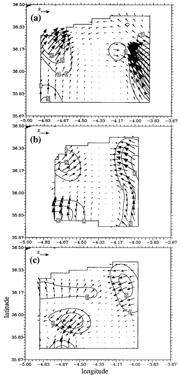
FIG. 14. Horizontal distribution at z = -100 m of the vertical advection of horizontal velocity by the QG vertical velocity ( w^{\text{QG}} \mathbf{u}_z ) for (a) survey 1, (b) survey 2, and (c) survey 3. Reference vector is 2 \times 10^{-6} \text{ m s}^{-2} . Only every other vector has been plotted. Isolines indicate the magnitude |w^{\text{QG}} \mathbf{u}_z| with \Delta = 1 \times 10^{-6} \text{ m s}^{-2} .
