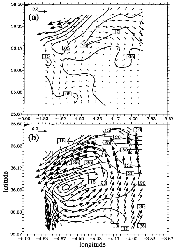
FIG. B1. Horizontal distribution at z = -13 m of the local acceleration field \Delta\mathbf{u}/\Delta t computed by differencing the current data in surveys 1 and 2 (a) and surveys 2 and 3 (b). Reference vector is 0.2 \times 10^{-5} \text{ m s}^{-2} . Only every other vector has been plotted. Isolines indicate the magnitude |\Delta\mathbf{u}/\Delta t| with \Delta = 0.05 \times 10^{-5} \text{ m s}^{-2} .
