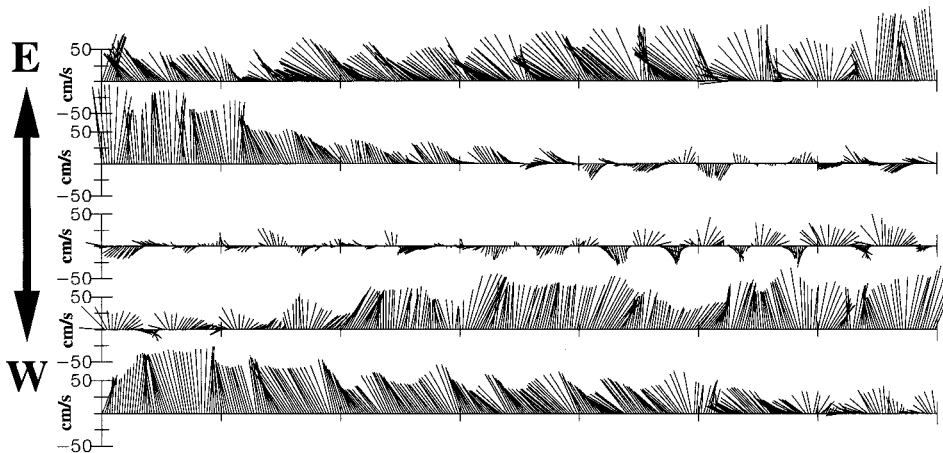
FIG. 20. Time series (five consecutive weeks with a sampling interval of 5 minutes) of the current meter 151 [positioned at 67-m depth on 36^{\circ}01.5'N , 4^{\circ}43.9'W (see Fig. 1a)]. During the third week the AJ current was not present in the current meter location [see Perkins et al. (1990) for detailed information]. Ticks interval is 1 day. The vertical axis is aligned with the east. Time interval between vectors is 30 minutes.
