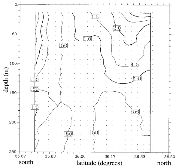
FIG. 18. Distribution at vertical section F for survey 1 (referenced in Fig. 1) of the magnitude of the gradient imbalance |\mathbf{I}_1| . \Delta = 0.5 \times 10^{-5} \text{ m s}^{-2} .
