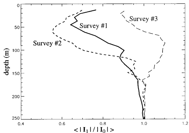
FIG. 19. Vertical dependence of the averaged ratio between the imbalances \langle |\mathbf{I}_1|/|\mathbf{I}_0| \rangle for the three surveys.
