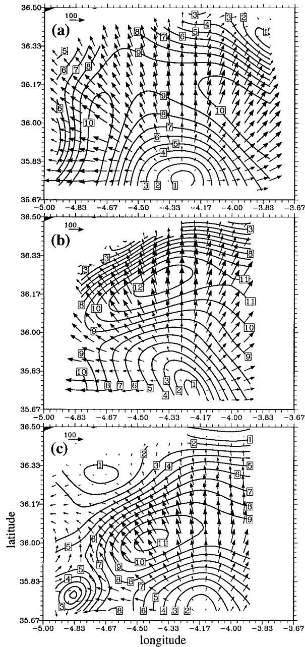
FIG. 11. Horizontal distribution at z = -13 m of the Coriolis acceleration field f\mathbf{k} \times \mathbf{u} for (a) survey 1, (b) survey 2, and (c) survey 3. Reference vector is 10 \times 10^{-5} \text{ m s}^{-2} . Only every other vector has been plotted. Isolines indicate the magnitude |f\mathbf{k} \times \mathbf{u}| with \Delta = 1 \times 10^{-5} \text{ m s}^{-2} .
