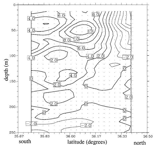
FIG. A1. Horizontal divergence ( \nabla \cdot \mathbf{u} ) distribution at vertical section F for survey 1 (referenced in Fig. 1). The dots indicate the interpolated ADCP data; \Delta = 2 \times 10^{-6} \text{ s}^{-1} .
