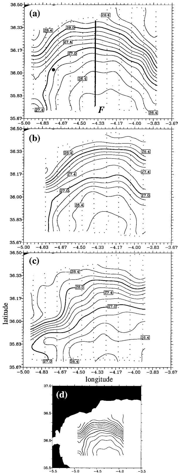
FIG. 1. Potential density ( \sigma_\theta ) distribution at z = -100 m for the three consecutive surveys [(a) survey 1, (b) survey 2, and (c) survey 3 respectively on 1–4, 6–8, and 9–11 Oct 1996]. Dots indicate the
