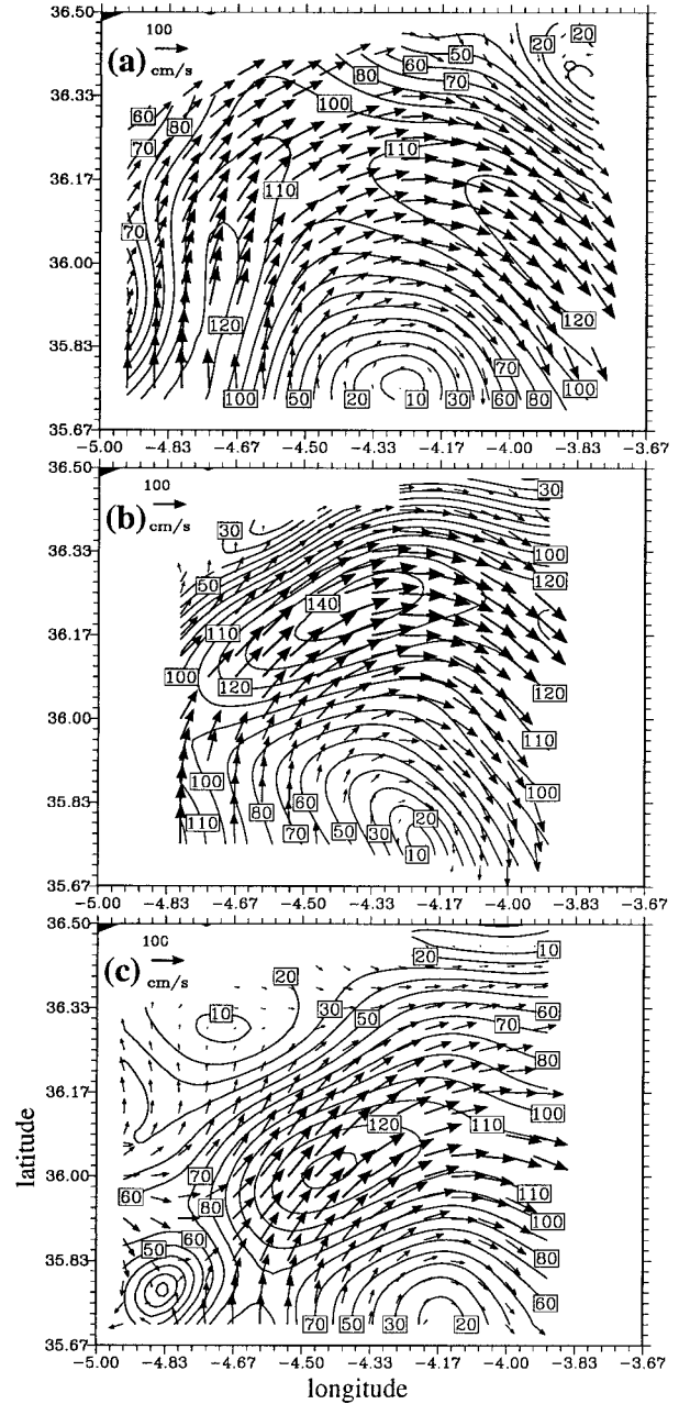
FIG. 8. Horizontal distribution at z = -13 m of \mathbf{u} (the interpolated ADCP velocity field) for (a) survey 1, (b) survey 2, and (c) survey 3. Reference vector is 100 \text{ cm s}^{-1} . For clarity only every other vector has been plotted. Isolines indicate the speed u \equiv |\mathbf{u}| with \Delta = 10 \text{ cm s}^{-1} .
