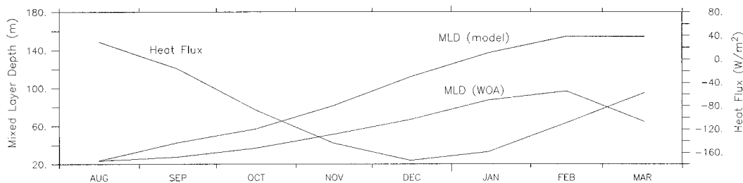
FIG. 2. Seasonal cycle (averaged along 28.5°N, 149.5°E–130.5°W) of net heat flux from da Silva et al. (1994), mixed layer depth calculated from the World Ocean Atlas 1994, and mixed layer depth calculated by the model.
