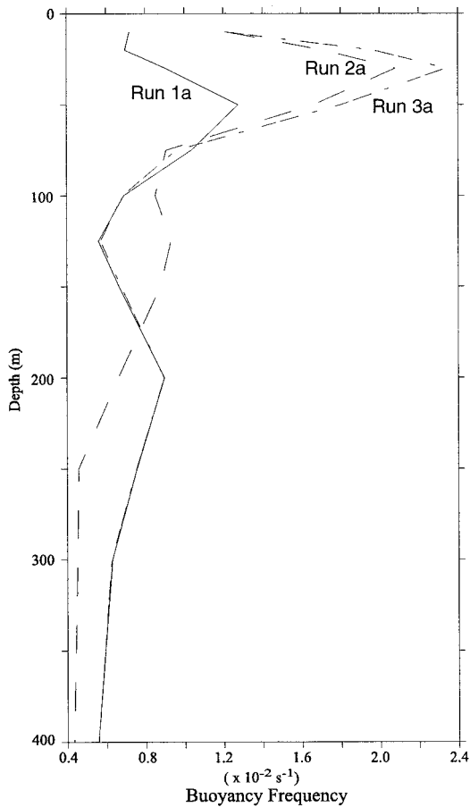
FIG. 9. Profiles of initial buoyancy frequency (in \text{s}^{-1} ) for the three test runs (solid: run 1a; dashed: 2a; and dashed-dotted: 3a).
