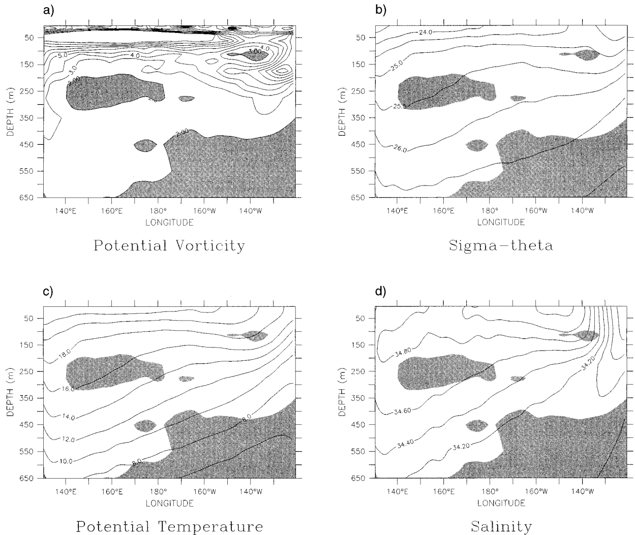
FIG. 4. Annual-mean climatological sections along 29.5°N derived from the World Ocean Atlas 1994. Local PV minima discussed in the text are shaded. (a) Potential vorticity (contour interval: 1 \times 10^{-10} \text{ m}^{-1} \text{ s}^{-1} ). Contours larger than 10 \times 10^{-10} \text{ m}^{-1} \text{ s}^{-1} are not displayed. (b) \sigma_\theta (contour interval: 0.5 \text{ kg m}^{-3} ). (c) Potential temperature (contour interval: 2^\circ\text{C} ). (d) Salinity (contour interval: 0.2 \text{ psu} ).
