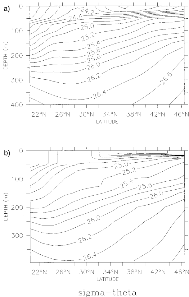
FIG. 7. August \sigma_\theta along 140.5^\circ\text{W} (contour interval = 0.2 \text{ kg m}^{-3} ). (a) Calculated from the World Ocean Atlas 1994. (b) Resulting from the model run discussed in the text.
