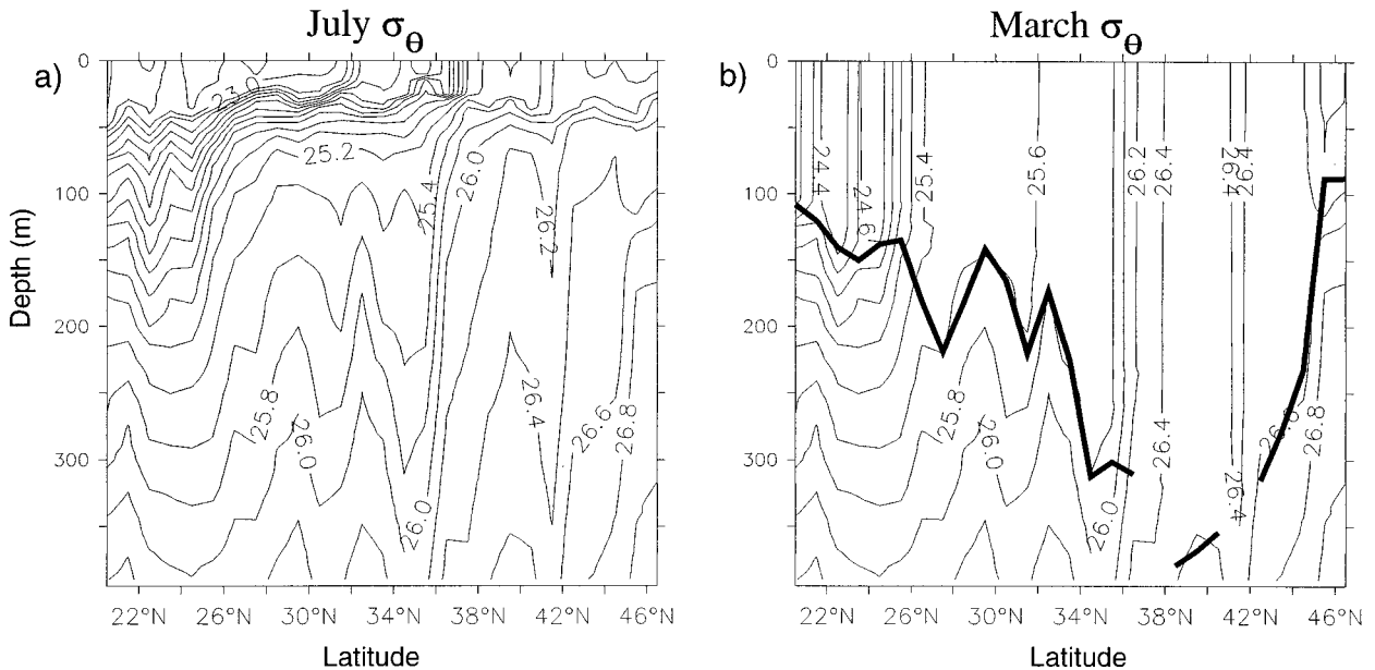
FIG. 13. Plot of \sigma_\theta along 179°E (contour interval: 0.2 kg m -3 ) (a) from WOCE P14N data in Jul 1993 and (b) resulting Mar density field from model run that was initialized with WOCE P14N data. The bold line shows mixed layer depth (defined as the depth at which \sigma_\theta is 0.125 kg m -3 different from the sea surface).
