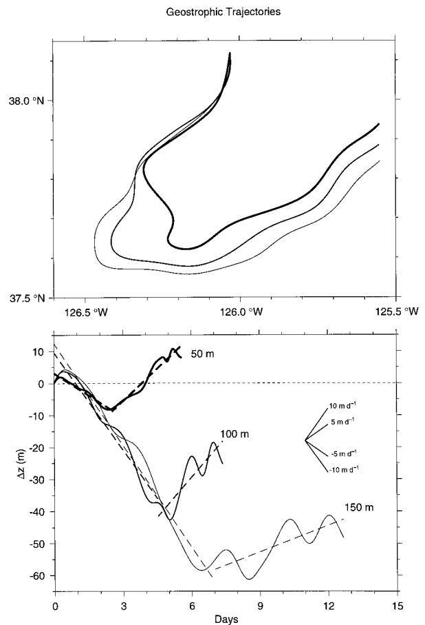
FIG. 14. Plots of geostrophic trajectories and net vertical displacements. Three geostrophic trajectories started at the same horizontal location (38.12°N, 126.03°W) but separated by 50 m in the vertical (50, 100, and 150 m) are shown in the upper panel. The net vertical excursions along those streamlines are shown in the lower panel. Different starting locations are indicated by line thickness. Lines fit using least squares to the upstream and downstream portions of the data are shown dashed.
