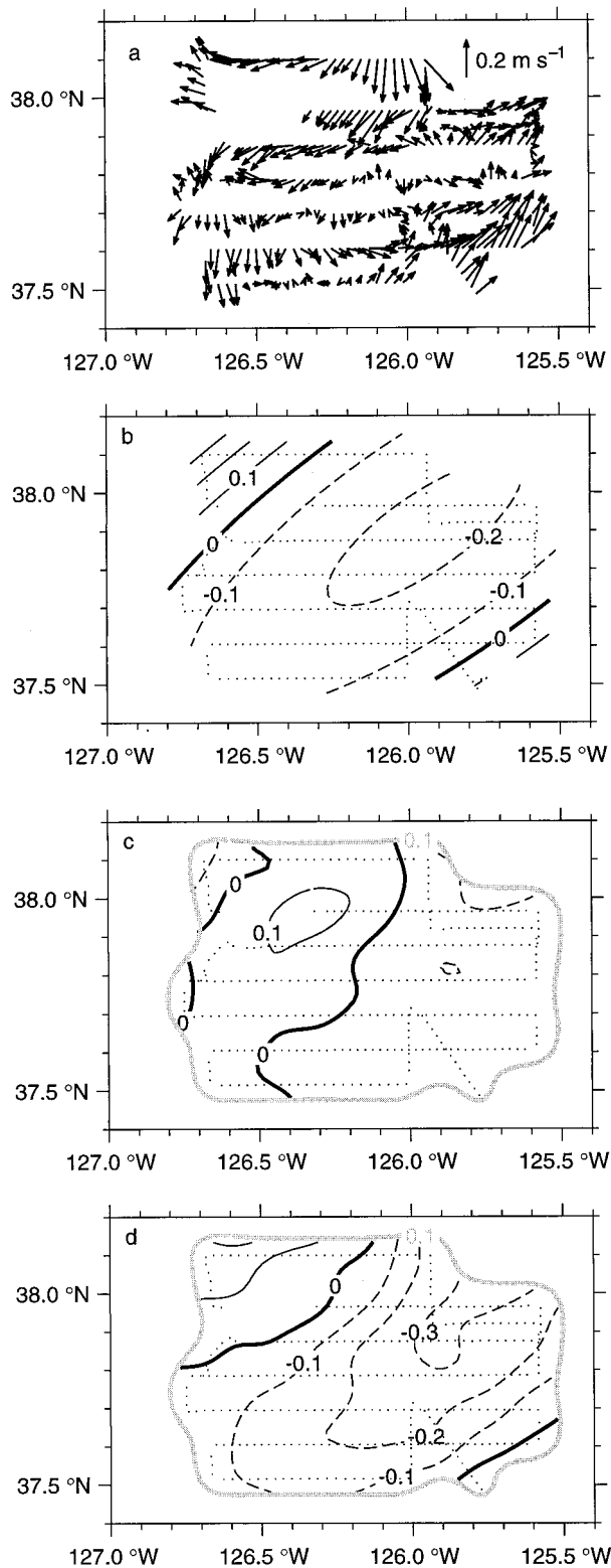
FIG. 7. Data reduction process for ADCP data at 200 m: (a) raw ADCP velocity vectors, (b) fitted nondivergent mean streamfunction ( \text{m}^2 \text{s}^{-2} ), (c) objectively analyzed residual streamfunction, and (d) total interpolated streamfunction. The streamfunctions as shown have been scaled by f and are equivalent to dynamic height. The bottom two panels also show the 0.1 error covariance contour.
