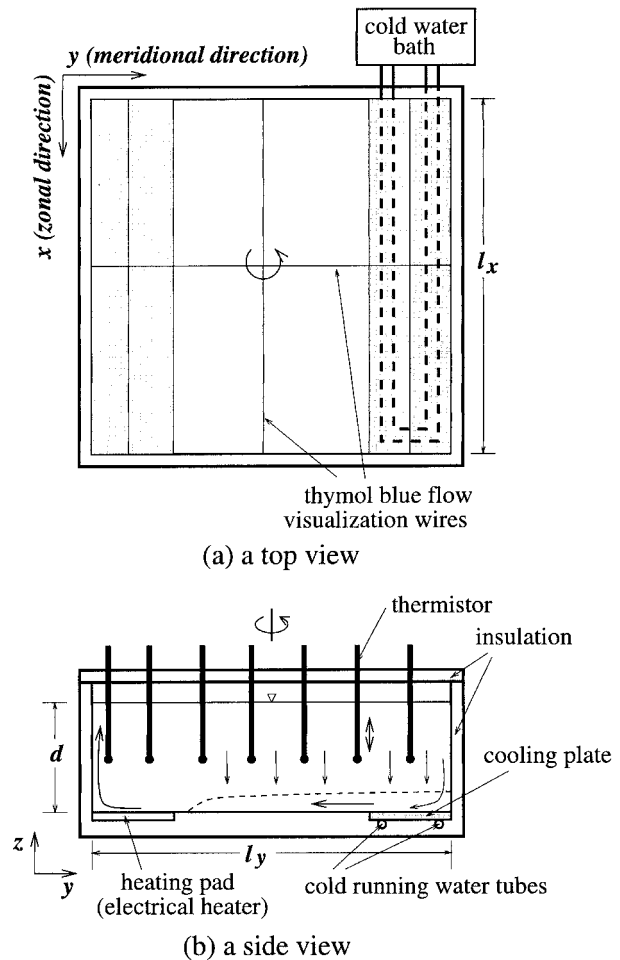
FIG. 1. The design of the experiment: (a) a top view and (b) a side view along a meridional section. The tank is 100 cm \times 100 cm \times 20 cm. The thermal forcing was applied using an electrical heater and a cooling plate along the bottom of the tank. The configuration is equivalent to an upside-down f -plane ocean with constant heat flux at the bottom.
