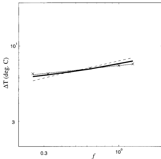
FIG. 7. Plot of \Delta T vs f when H_N = 50 \text{ W} . The experimental results are shown using "x." The thin solid line (slope = 0.13) is the least squares fit to the data. The dashed line (slope = 1/4 ) is for the geostrophic scaling law. The thick solid line (mean slope = 0.17) is for the corrected scaling law discussed in section 4d. A proportionality constant of about 3 was applied to fit the scaling laws to the data.
