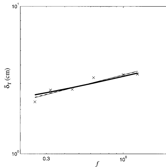
FIG. 8. Plot of \delta_T vs f when H_N = 50 \text{ W} . The experimental results are shown using "x." The thin solid line (slope = 0.29) is the least squares fit to the data. The dashed line (slope = 1/4 ) is for the geostrophic scaling law. The thick solid line is for the corrected scaling law discussed in section 4d.
