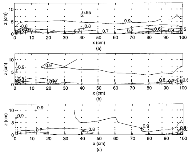
FIG. 6. Zonal temperature sections when f = 1 \text{ s}^{-1} and H_N = 50 \text{ W} (a) y = 70 \text{ cm} , (b) y = 50 \text{ cm} , and (c) y = 30 \text{ cm} .
