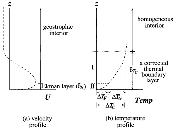
FIG. 9. Schematic profiles of (a) velocity and (b) temperature.
