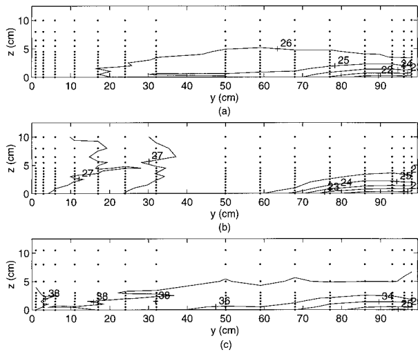
Fig. 2. Meridional temperature sections at x = 50 cm with (a) f = 0.63 s ^{-1} and H_N = 50 W, (b) f = 1 s ^{-1} and H_N = 50 W, and (c) f = 1 s ^{-1} and H_N = 200 W. The meridional wall to the left when looking toward the cold end is at x = 0 cm and is equivalent to the eastern boundary of the oceans. The dots indicate the location of temperature measurements. The heating plate is 0 cm \leq y \leq 20.3 cm and the cooling plate is 79.7 cm \leq y \leq 100 cm.
