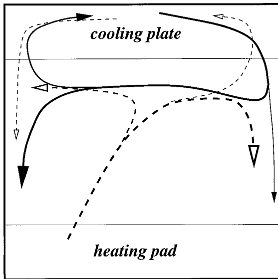
FIG. 4. A schematic diagram of flow pattern. A solid curve represents cold current and a dotted curve represents warm current. If a solid curve and a dotted curve are stacked, the cold flow is near the bottom and warm flow is above the cold flow.
