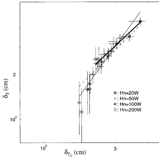
FIG. 11. Comparison of the corrected scaling law \delta_{Tc} and the experimental results \delta_T . The dashed line is from the geostrophic scaling law with a proportionality constant, 1.0. The thin solid line is the least squares fit of all the data and the thick solid line is the least squares fit of \delta_{T_{exp}} > 2 cm.
