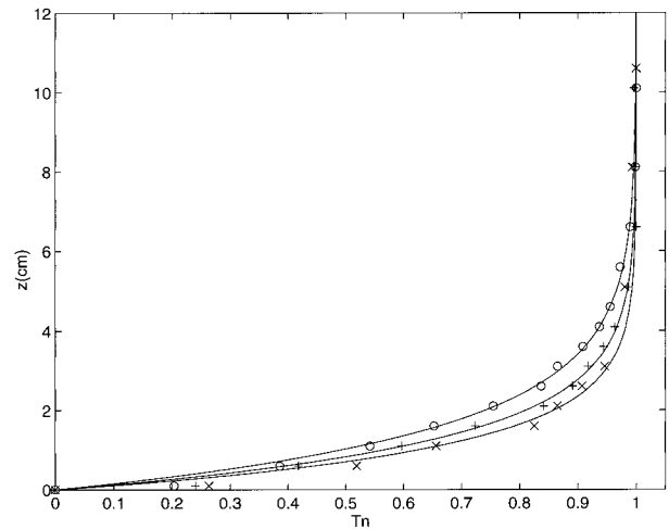
Fig. 3. Normalized temperature profiles at (x, y) = (49.5 cm, 96 cm) ( \circ : f = 1.25 s ^{-1} , H_N = 50 W; + : f = 0.45 s ^{-1} , H_N = 50 W; \times : f = 1.25 s ^{-1} , H_N = 200 W). Solid curves are the least square fits of profiles to exponential functions.
