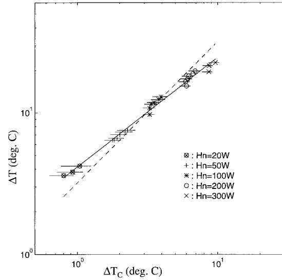
FIG. 10. Comparison of \Delta T_C(f, H) from the corrected scaling law and the experiment. The dashed line is from the scaling law with a proportionality constant 2.7. The solid line is the least squares fit of the experimental data.
