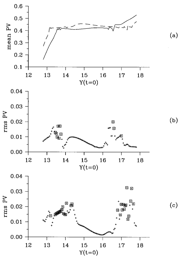
FIG. 15. Lagrangian potential vorticity statistics for case III. (a) Mean potential vorticity vs initial meridional location, Y(t = 0) , for the western transect (plotted with the solid line) and eastern transect (plotted with the dashed line) shown in Fig. 13b. (b) Standard deviation vs initial meridional location for the western transect. Particle trajectories that exhibit rapid potential vorticity transitions ( \Delta q > 0.015 over 10 time units) have their rms data point augmented with a square. (c) As in (b) but for the eastern transect.
