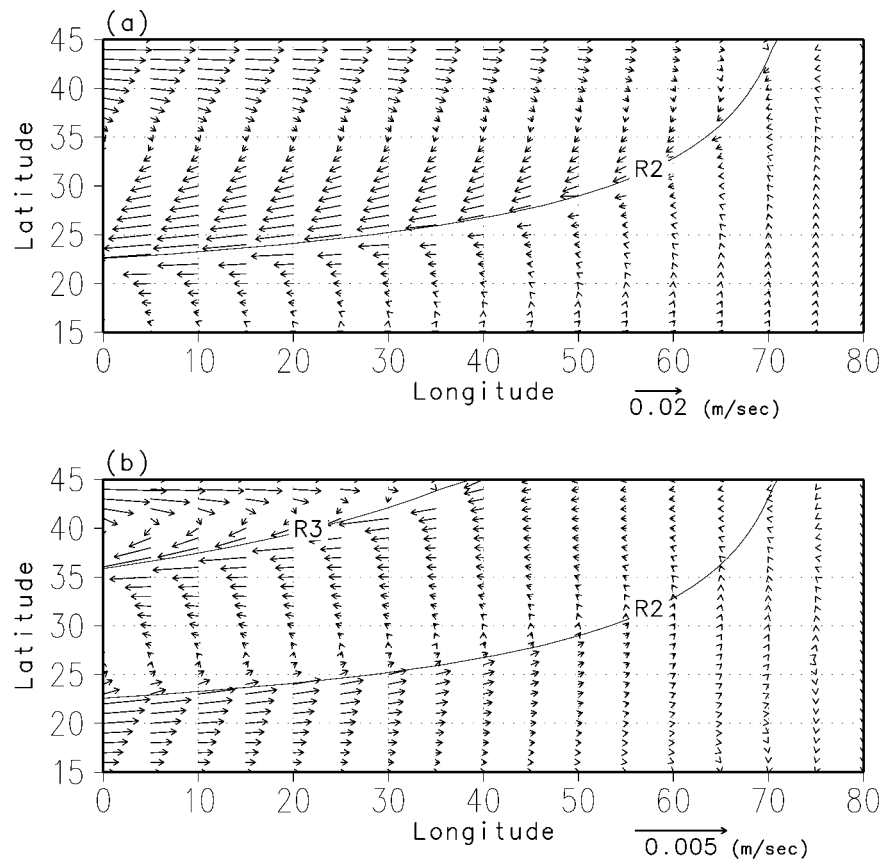
FIG. 4. Velocity fields obtained from the model in (a) the upper intermediate layer, and (b) the lower intermediate layer. In the region north of the curve R2 (R3), potential vorticity is homogenized in the upper (lower) intermediate layer.
