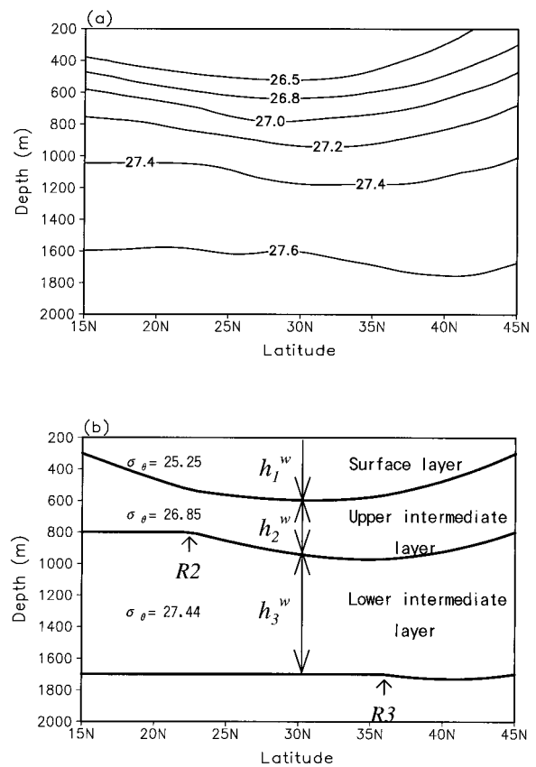
FIG. 2. Meridional cross sections of (a) observed density surfaces along the date line, and (b) modeled layer interfaces at a location equivalent to the date line. The distance from this location to the eastern boundary of the model is taken as 80°, which is approximately equivalent to the distance between the date line and the coast of North America. The observed density distribution is based on the climatological data of Levitus et al. (1994) and Levitus and Boyer (1994b). The model is similar to that proposed by Pedlosky and Young (1983), but ventilated layers in their model are simplified into one layer. Details of the model description are given in section 2a, in terms of layer thicknesses of h_1^w , h_2^w , and h_3^w . In (a), contours in the surface layer less than 26.5 \sigma_\theta are omitted to avoid crowding. In (b), R2 (R3) represents the position of the southern boundary of the potential vorticity homogenized region in the upper (lower) intermediate layer.
