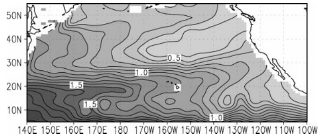
FIG. 8. Concentration of dissolved oxygen ( \text{ml L}^{-1} ) along the density surface of 27.4 \sigma_\theta . The density surface lies within the lower intermediate layer ( 27.2 – 27.67 \sigma_\theta ) of the North Pacific.
