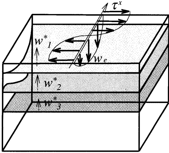
FIG. 3. Schematic representation of the 3\frac{1}{2} -layer model. Ekman pumping, w_e , is given by the curl of wind stress, \tau^x . Diapycnal flows, w_1^* , w_2^* , and w_3^* , are taken into account as the forcing accompanied by the thermohaline process of diapycnal advective–diffusive density balance.
