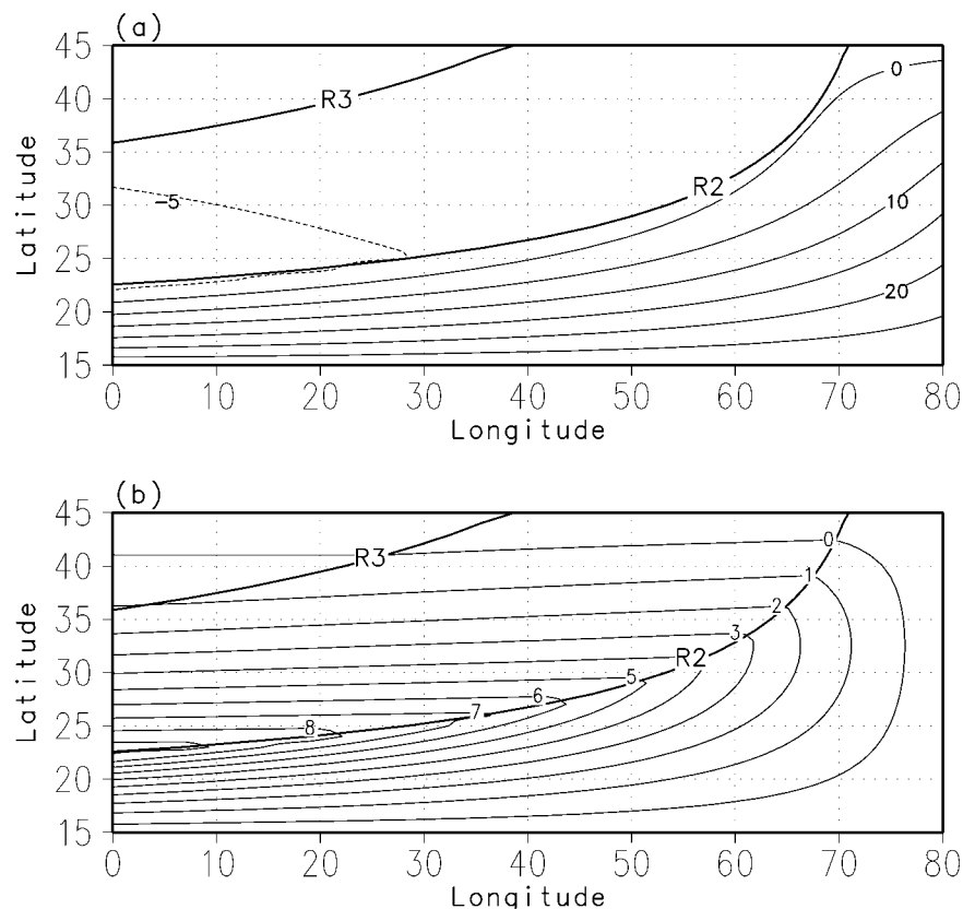
FIG. 5. Divergence fields of diapycnal velocity in (a) the upper intermediate layer and (b) the lower intermediate layer. Values in the fields are given as (a) w_1^* - w_2^* and (b) w_2^* - w_3^* . The units of the contour labels are 10^{-8} \text{ m s}^{-1} , and the contour intervals are 5 \times 10^{-8} and 1 \times 10^{-8} \text{ m s}^{-1} for (a) and (b), respectively. The two curves, R2 and R3, are the same as those shown in Fig. 4.
