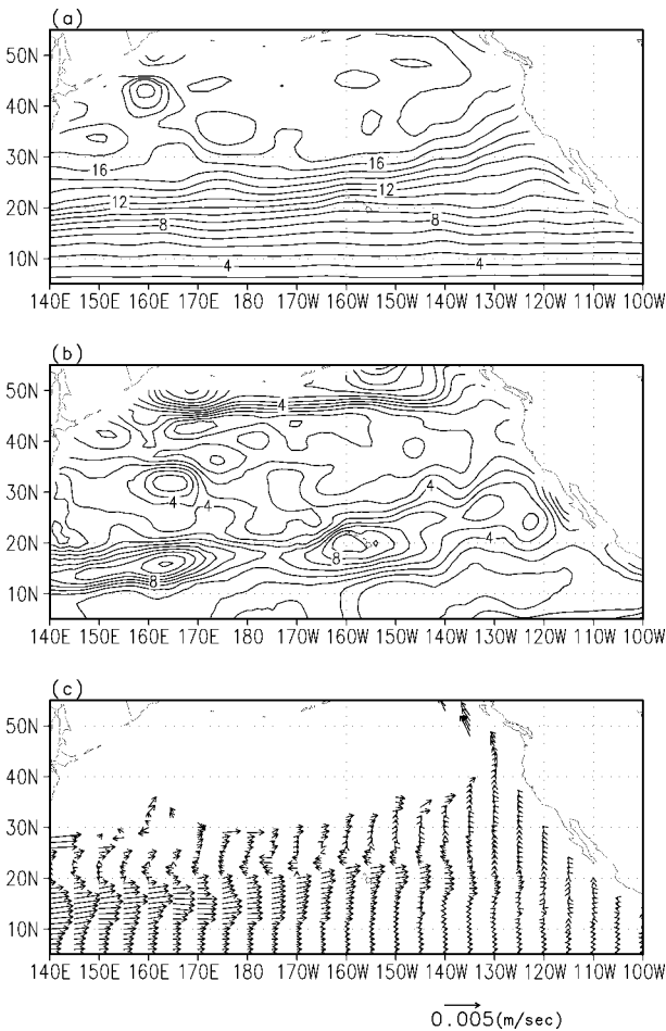
FIG. 7. Distributions of (a) potential vorticity in the layer defined by the density surfaces of 27.2 and 27.5 \sigma_\theta in the North Pacific, (b) the difference of diapycnal velocities between the upper and lower interfaces of the layer, and (c) current velocity averaged in the layer caused by the divergence of diapycnal velocity. In (a) values of potential vorticity are calculated by dividing the Coriolis parameter by the layer thickness. The units of the contour labels are 10^{-8} \text{ m}^{-1} \text{ s}^{-1} , and the contour interval is 1 \times 10^{-8} \text{ m}^{-1} \text{ s}^{-1} . The contours correspond to the characteristic paths to obtain the velocity field in (c). In (b) the units of the contour labels are 10^{-8} \text{ m} \text{ s}^{-1} , and the contour interval is 1 \times 10^{-8} \text{ m} \text{ s}^{-1} . In (c) the region where the velocity vectors are not shown is sheltered from the penetration of characteristic paths from the eastern boundary. Therefore, in this region, the solution of the currents cannot be obtained.
