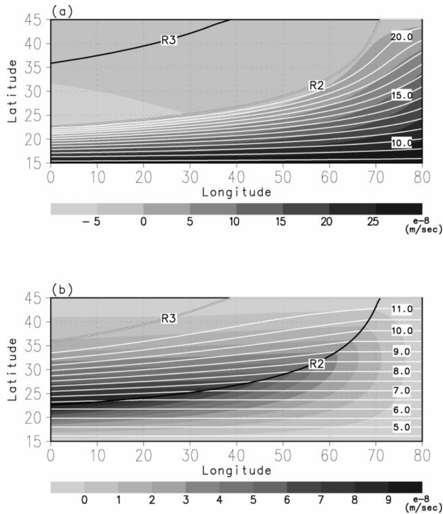
FIG. 6. Characteristic paths (white contours) and divergence fields of diapycnal velocity (shades) in (a) the upper intermediate layer, and (b) the lower intermediate layer. The characteristic paths are given as curved or straight lines of f/h_2^w = \text{const} and f/h_3^w = \text{const} in the upper and lower intermediate layers, respectively. The units of the contour labels are 10^{-8} \text{ m}^{-1} \text{ s}^{-1} , and the contour intervals are 1 \times 10^{-8} and 0.5 \times 10^{-8} \text{ m}^{-1} \text{ s}^{-1} for (a) and (b), respectively. The divergence fields of diapycnal velocity shown in Fig. 5 are superimposed with shading. Darker (lighter) shades represent larger (smaller) divergence.
