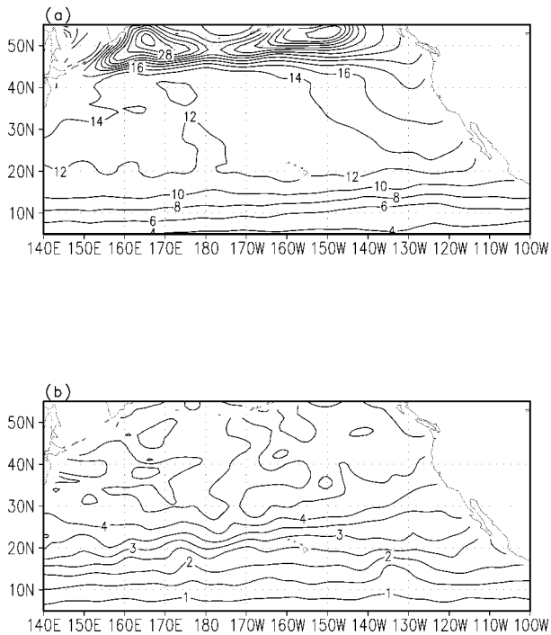
FIG. 1. Distributions of potential vorticity in the North Pacific along isopycnal surfaces of (a) 26.8 and (b) 27.4 \sigma_\theta . Values of potential vorticity are calculated as -\rho^{-1}f\partial\rho/\partial z , where \rho is density and f is the Coriolis parameter. The density field is obtained from climatological data of temperature (Levitus and Boyer 1994b) and salinity (Levitus et al. 1994). Units of the contour labels are 10^{-11} \text{ m}^{-1} \text{ s}^{-1} , and the contour intervals are 2 \times 10^{-11} and 0.5 \times 10^{-11} \text{ m}^{-1} \text{ s}^{-1} for (a) and (b), respectively.
