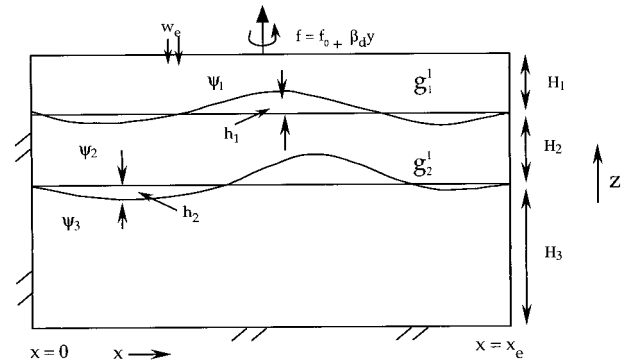
FIG. 1. A three-layer configuration is shown. The model is flat bottomed, forced by a variable wind, and on a \beta plane. Notation is standard.
