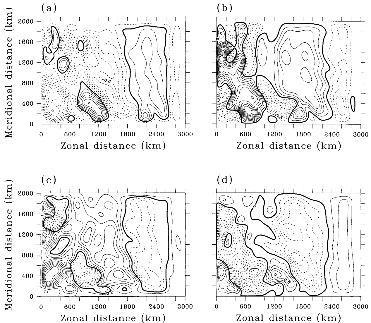
FIG. 8. As in Fig. 3 but using a six-layer QG model.
