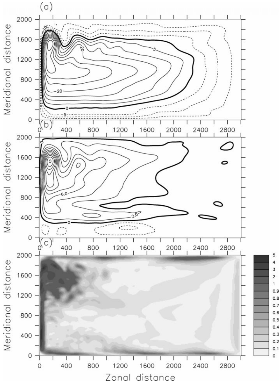
FIG. 2. Mean state circulation: (a) upper-layer streamfunction averaged over the last 12 years of our three-layer experiment (units are 10^3 \text{ m}^2 \text{ s}^{-1} ); (b) second-layer streamfunction, so averaged (units are 10^3 \text{ m}^2 \text{ s}^{-1} ); (c) eddy kinetic energy from the upper layer, so averaged (units are \text{m}^2 \text{ s}^{-2} ).
