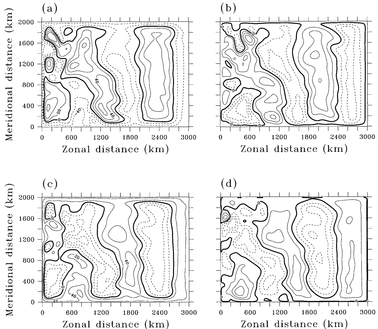
FIG. 3. First baroclinic mode wave propagation at fixed phases, and averaged over the last 12 years of our three-layer experiment: (a) at the point of maximum Ekman pumping, (b) three months later than (a), (c) at the point of minimum Ekman pumping, and (d) three months later than (c).
