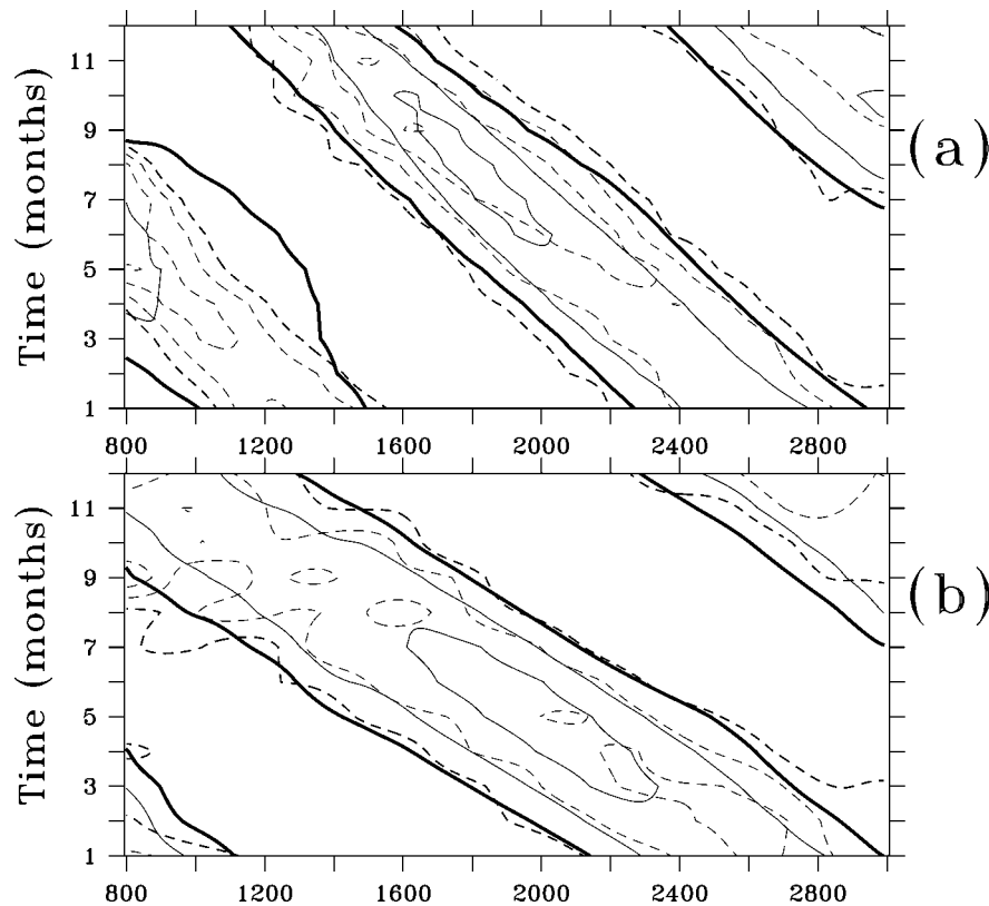
FIG. 9. Time-longitude plots comparing the three-layer model (solid) to the six-layer model (dashed): (a) Y = 500 km and (b) Y = 1400 km. The zonal average of the data has been removed.
