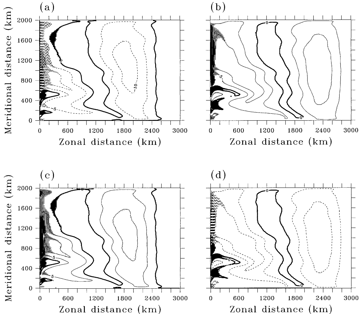
FIG. 4. As in Fig. 3 but using the asymptotic theory in (5).
