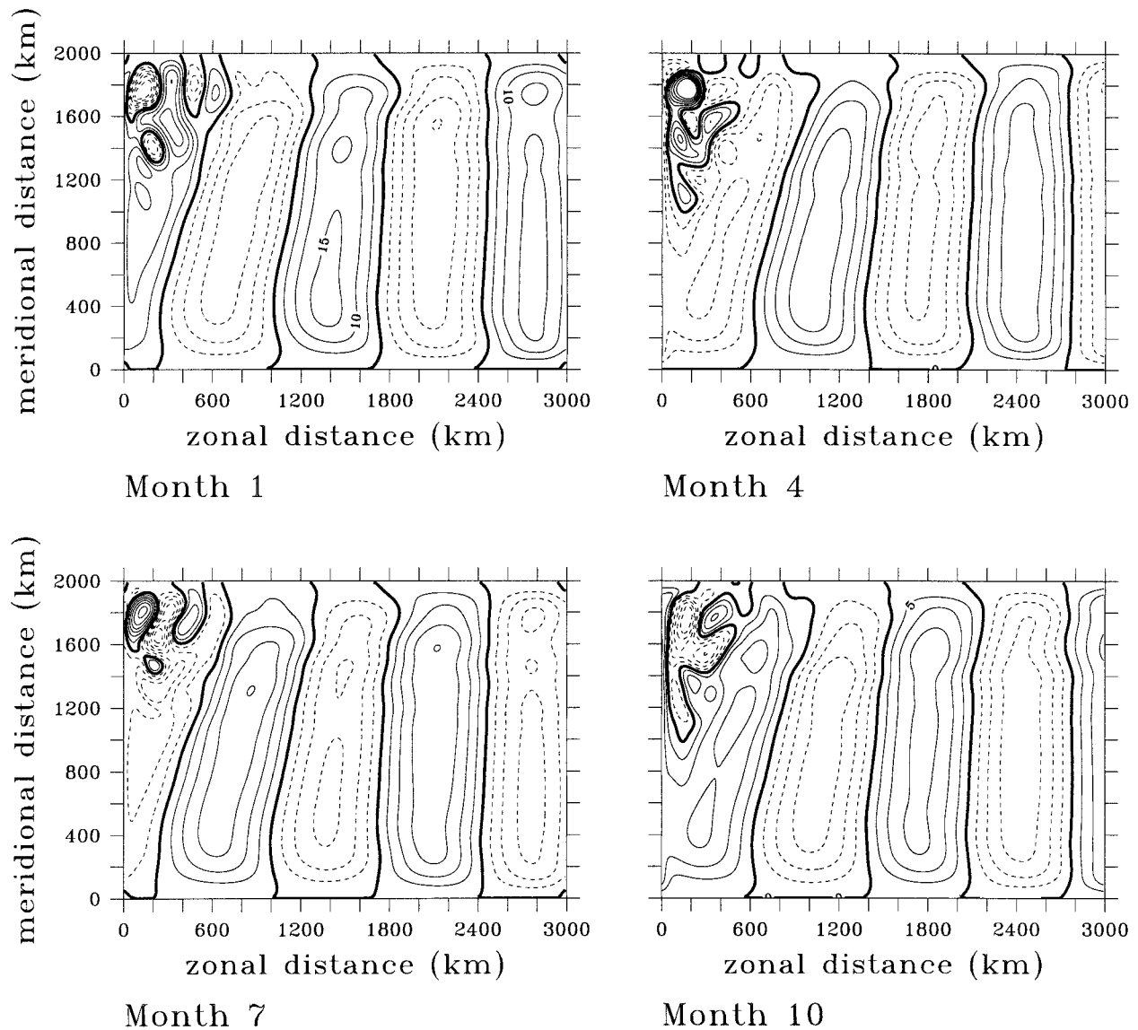
FIG. 7. As in Fig. 3 but using a two-layer QG model.
