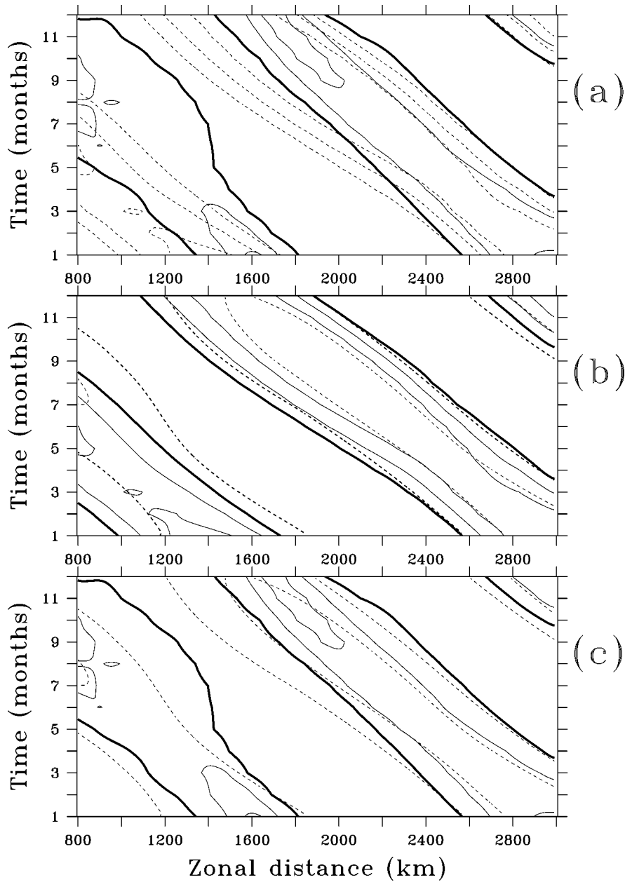
FIG. 6. As in Fig. 5 but at Y = 500 km.
