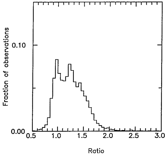
FIG. 5. A histogram of the ratio of planetary-wave phase speed calculated by the Killworth et al. (1997) method including mean vertical shear, to Rossby wave phase speed obtained by neglecting mean shear (Chelton et al. 1998) for 1^\circ \times 1^\circ squares over all ocean basins, 10^\circ\text{--}50^\circ\text{S} , 10^\circ\text{--}50^\circ\text{N} .
