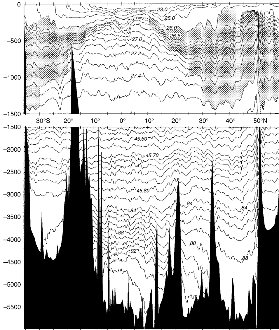
FIG. 2. Potential density ( \sigma_n referenced to 0 dbar above 1500 m, \sigma_t referenced to 4000 dbar below 1500 m) along 179°E in the western Pacific. Note the northward–upward isopycnal slopes near surface; northward–downward slopes at middepth. The hatched region corresponds to the range over which Keffer’s (1985) maps show potential vorticity approximately homogeneous on isopycnal surfaces.
