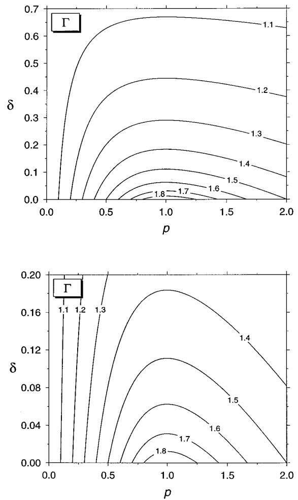
FIG. 4. The speedup ratio c/c_1 for zero interior potential vorticity gradient as a function of parameters p, \delta , depending on density difference ratio r and mean layer depths D_1, D_2, D_3 .
