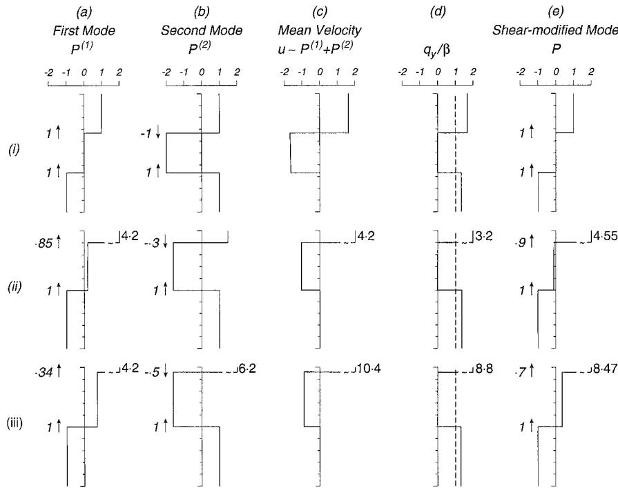
FIG. 3. Features of three example calculations with the three-layer model using the parameter settings in columns (i), (ii), and (iii) of Table 1. For the standard case (no shear) the first- (a) and second-mode (b) vertical profiles of pressure are shown (arbitrary units). The interfacial vertical velocities of the modes are indicated on these panels by arrows with accompanying numerical magnitudes, relative to W_2 = 1 . (c) Mean velocity profiles constructed from first and second modes with zero mean and zero bottom velocity (unit: \text{cm s}^{-1} ); and (d) associated meridional potential vorticity gradients (scaled by \beta ). (e) The shear-modified pressure modes for (c) and (d) (arbitrary units); interfacial vertical velocities are indicated.
