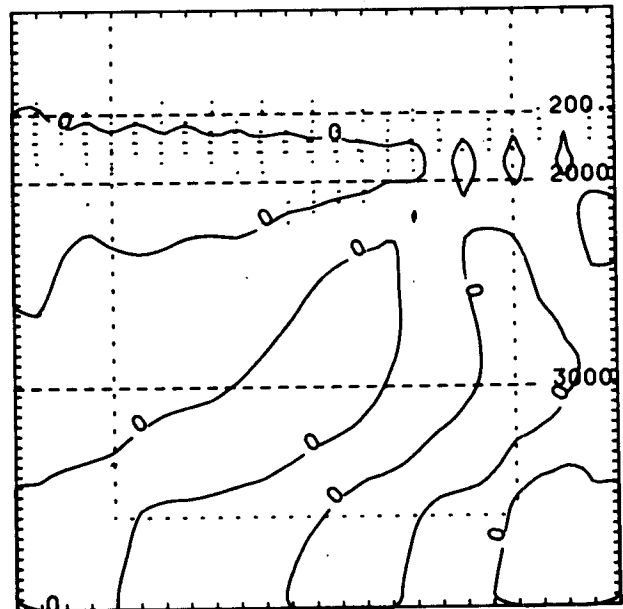
FIG. 5. As in Fig. 2 except generated by a source on the slope at 36 days.
