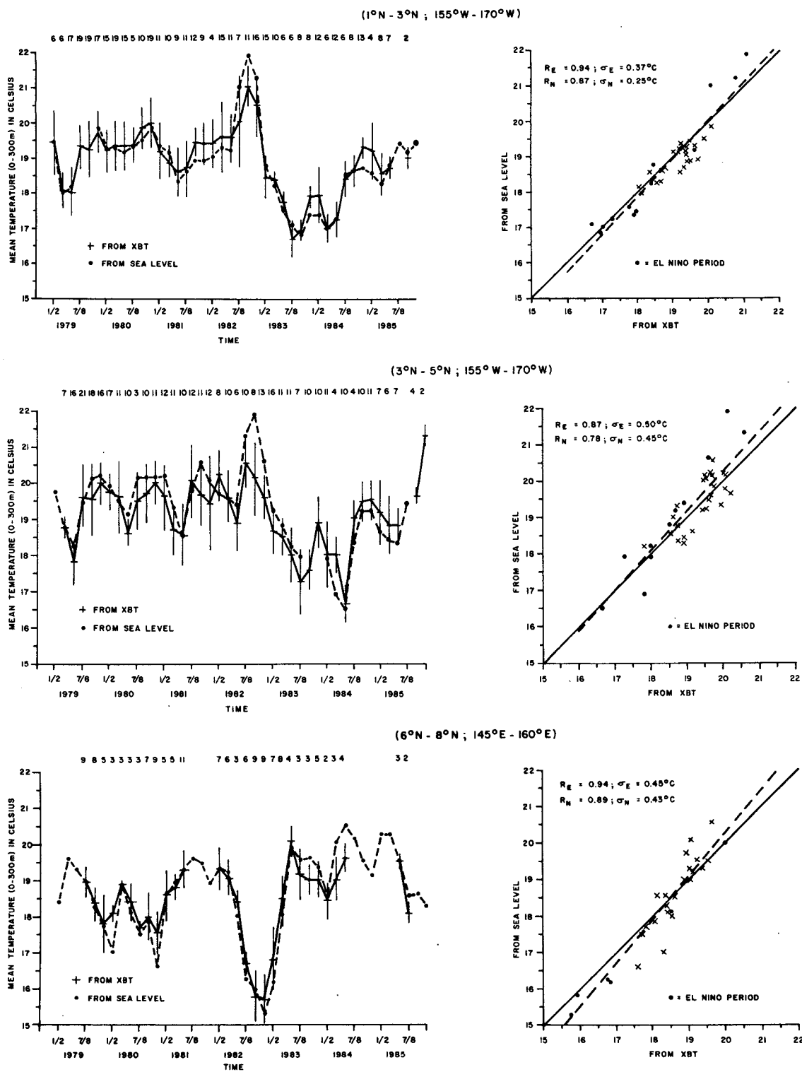
FIG. 5a. (left panel) Comparison between 2-month-averaged XBT heat content estimates \bar{T}(XBT) in the (1°N-3°N, 155°W-170°W) rectangles (solid lines) and the heat content derived from sea level recorded in Christmas Island \bar{T}(SL) (broken lines). The bars denote the standard deviations of \bar{T}(XBT) during the given period. The upper numbers are the numbers of XBT profiles used to calculate the heat content. (right panel) Regression analysis between the two heat content estimates \bar{T}(XBT) and \bar{T}(SL) . R_E , rms_E ( \sigma_E ) and R_N , rms_N ( \sigma_N ) are defined in Table 1.
