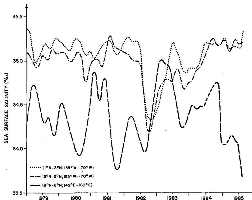
FIG. 6. Sea surface salinity variations in the reported rectangles during the 1979–85 period.
