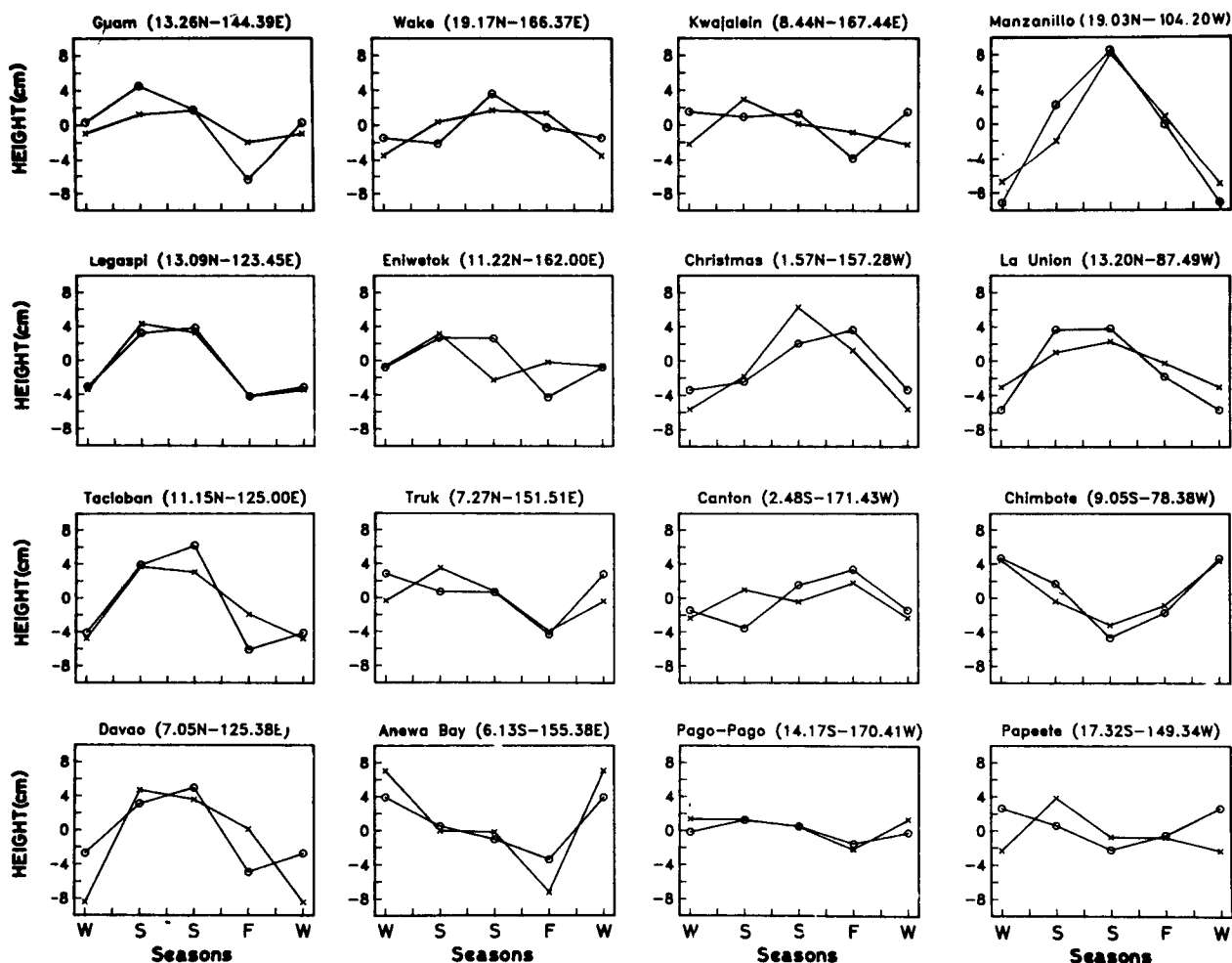
FIG. 2. Comparison between the seasonal steric level (ST(C1):X) and sea level (SL:O) variations 16 locations of the tropical Pacific Ocean. The errors in the sea level are 2 cm and those in the steric level about 25% of the seasonal signals. Winter (W) = Feb-Apr, etc.
