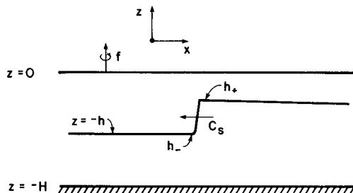
FIG. 6. Shock wave structure. Shock waves are coherent structures consisting of a balance between steepening and dissipation. The changes in fluid properties, in this case in h , can occur almost discontinuously. h_- refers to the thermocline thickness west of the shock, and h_+ refers to the thermocline thickness east of the shock. The shock propagation speed, c_s , can be computed from a knowledge of these parameters alone.
