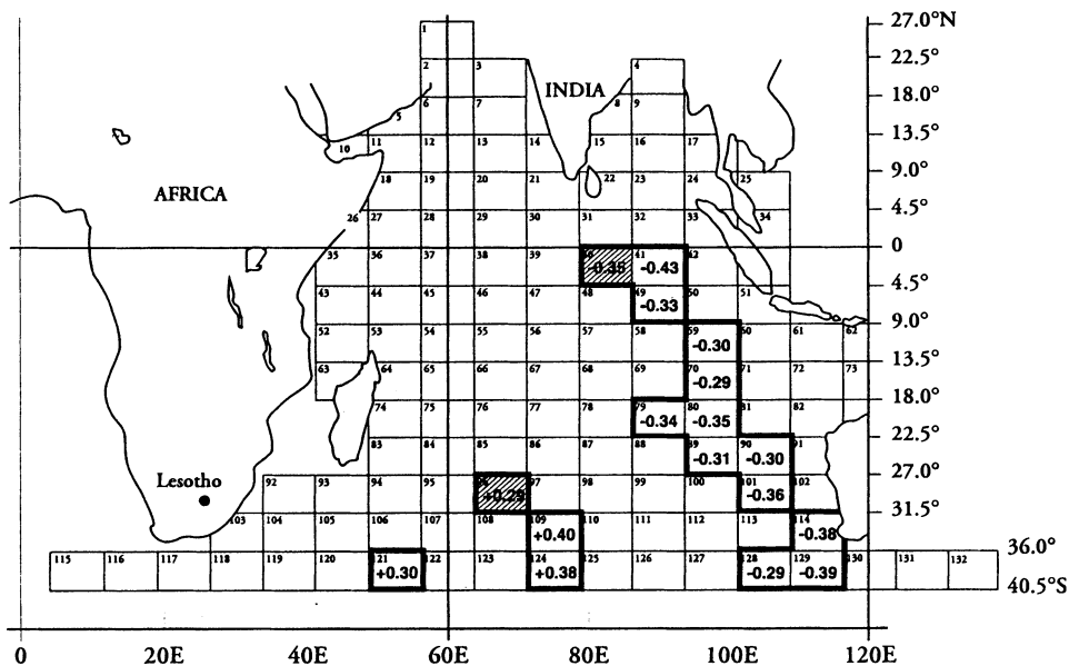
Fig. 6. Significant correlation between December SST and February rainfall in the Lesotho Lowlands. Legend: Shaded grid squares also have significant correlation between February SST and February rainfall.
