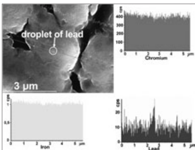
Figure 7. Image and line scanning on the interdentritic, cracked surface with droplets of lead
