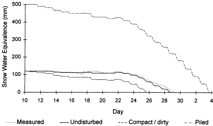
Fig. 4. Calculated SWE for the three snow types modelled against the measured values, April – May, 1993.
