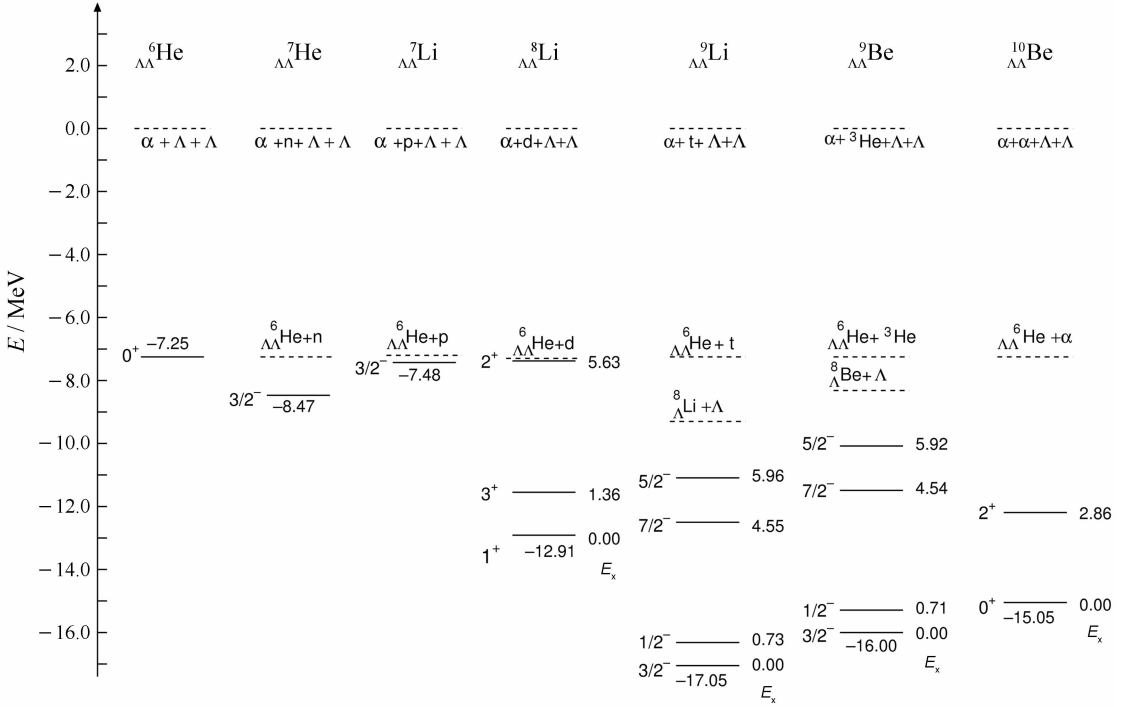
Fig. 3 Energy levels of double- \Lambda hypernuclei, {}_{\Lambda\Lambda}{}^6\text{He} , {}_{\Lambda\Lambda}{}^7\text{He} , {}_{\Lambda\Lambda}{}^7\text{Li} , {}_{\Lambda\Lambda}{}^8\text{Li} , {}_{\Lambda\Lambda}{}^9\text{Li} , {}_{\Lambda\Lambda}{}^9\text{Be} and {}_{\Lambda\Lambda}{}^{10}\text{Be} calculated using the \alpha+x+\Lambda+\Lambda model with x=0, n, p, d, t, {}^3\text{He} and \alpha , respectively.
