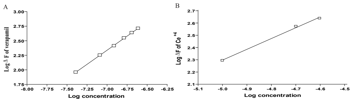
Figure 7. Stoichiometry of the reaction between VP and Ce (IV) adopting limiting logarithmic method. A, Log (VP) vs log Δ F; B, Log (Ce (IV)) vs log Δ F.
