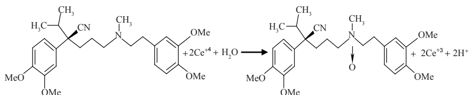
Figure 8. Proposal for the reaction between VP and Ce (IV).
