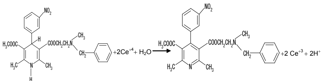
Figure 10. Proposal for the reaction between NC and Ce (IV).
