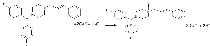
Figure 11. Proposal for the reaction between FZ and Ce (IV).
