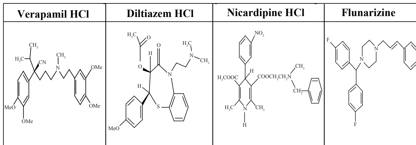
Figure 1. Structural formulae of the studied drugs.
