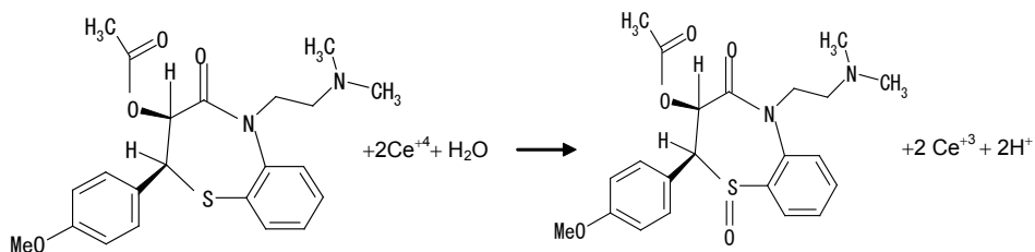
Figure 9. Proposal for the reaction between DLT and Ce (IV).
