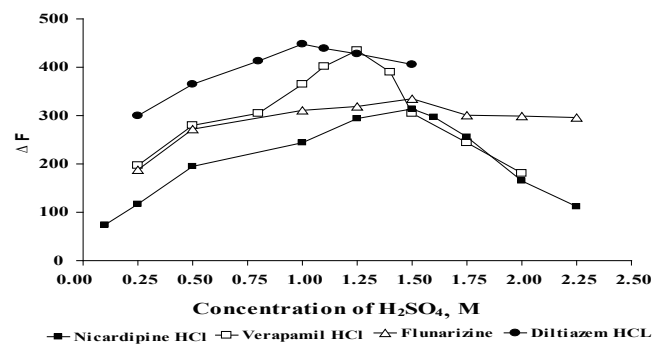
Figure 4. Effect of molar concentration of \text{H}_2\text{SO}_4 on the relative fluorescence intensity. ●, 0.06 \mu\text{g mL}^{-1} DLT; □, 0.1 \mu\text{g mL}^{-1} VP; △, 0.1 \mu\text{g mL}^{-1} FZ; ■, 0.1 \mu\text{g mL}^{-1} NC.
