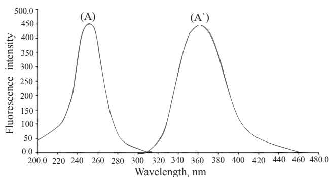
Figure 2. Excitation and emission spectra of induced Ce(III) by oxidation of 0.06 \mu\text{g mL}^{-1} DLT with Ce (IV) where: (A), Excitation spectrum; (A'), Emission spectrum.
