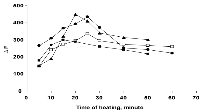
Figure 5. Effect of the heating time on the relative fluorescence intensity. \Delta , 0.06 \mu\text{g mL}^{-1} DLT; \bullet , 0.1 \mu\text{g mL}^{-1} VP; \square , 0.1 \mu\text{g mL}^{-1} FZ; \blacklozenge , 0.1 \mu\text{g mL}^{-1} NC.
