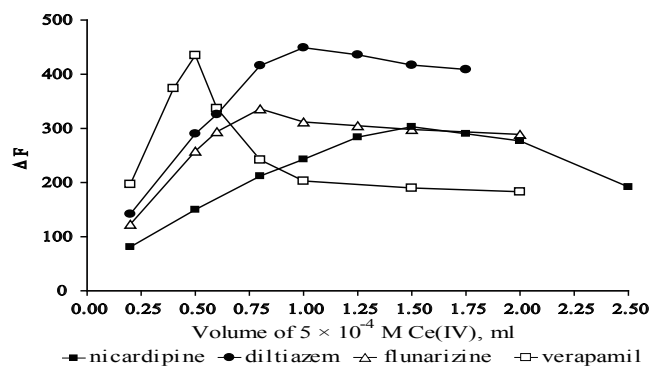
Figure 3. Effect of volume of 5 \times 10^{-4} M Ce (IV) on the relative fluorescence intensity. ●, 0.06 \mu\text{g mL}^{-1} DLT; □, 0.1 \mu\text{g mL}^{-1} VP; △, 0.1 \mu\text{g mL}^{-1} FZ; ■, 0.1 \mu\text{g mL}^{-1} NC.
