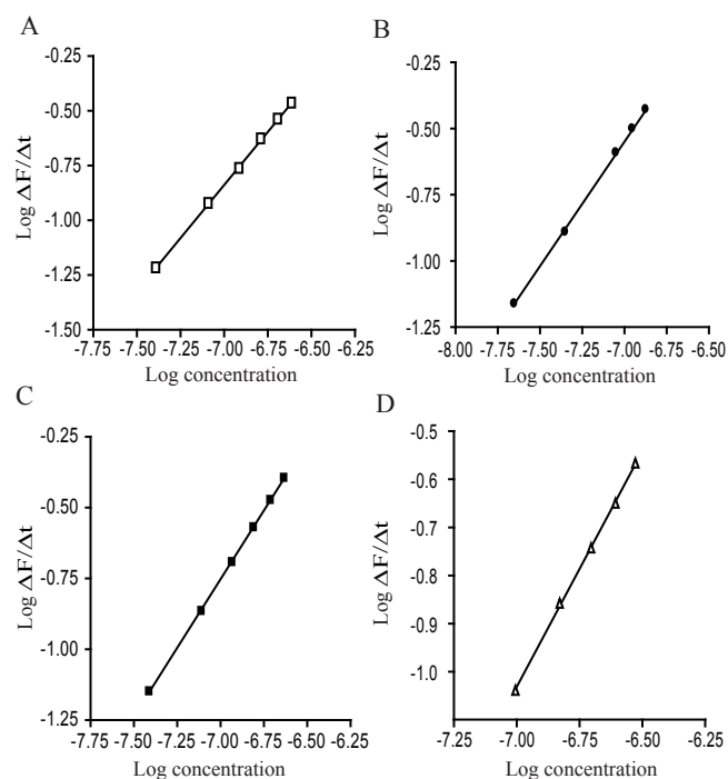
Figure 6. Plot of Log reaction rate (Log ΔF/Δt) versus Log concentration of: A, VP; B, DLT; C, NC; D, FZ.
