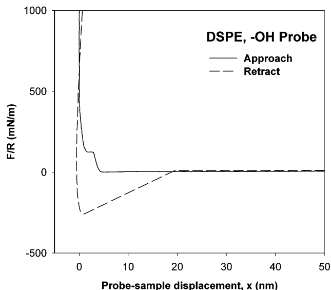
Figure 3. Normalized force ( F/R ) vs probe-sample displacement ( x ) curves for the indentation of DSPE/DSPE bilayers using -OH probes. A small jump-in (breakthrough) is observed on approach, and a strong adhesion on retract.
