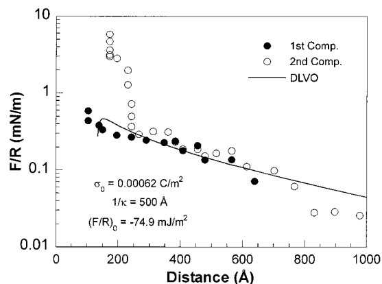
Figure 10. SFA force profiles for (C_{16})_2 -Glu-C 2 -GlyOME monolayers in pure water (pH 5.6). The force and adhesion data are very similar to those for the uncharged (C_{16})_2 -Glu-C 2 -Gly monolayers (Figure 5). OHP for the DLVO fits is set at D_0 + 15 Å to account for interpenetration.
