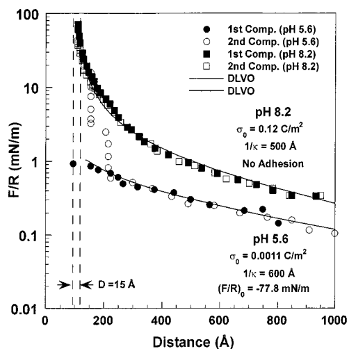
Figure 6. SFA force profiles for (C_{16})_2 -Glu- C_2 -Gly monolayers in pure water at pH 5.6 and 8.2. D_0 is 15 Å smaller at pH 5.6 than at pH 8.2. At pH 5.6, a large adhesion is measured, leading to the bilayer disruption observed on second compression. No adhesion or bilayer disruption is observed at pH 8.2. The contact bilayer thickness ( D_0 ) was 15 Å smaller in the adhesive case (pH 5.6), suggesting that headgroup interpenetration is occurring on contact. OHP for the pH 5.6 DLVO fit was shifted accordingly (see text).
