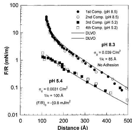
Figure 11. SFA force profiles for (C_{18})_2 -Glu-C 2 -COOH monolayers in 1 mM KBr, measured at the same spot (first at pH 8.3 and then at pH 5.4). For both fits, the OHP for DLVO fits was set to D = D_0 value measured at pH 8.3. Unlike the (C_{16})_2 -Glu-C 2 -Gly case (Figure 5), only a small pull-off force is observed at low pH.
