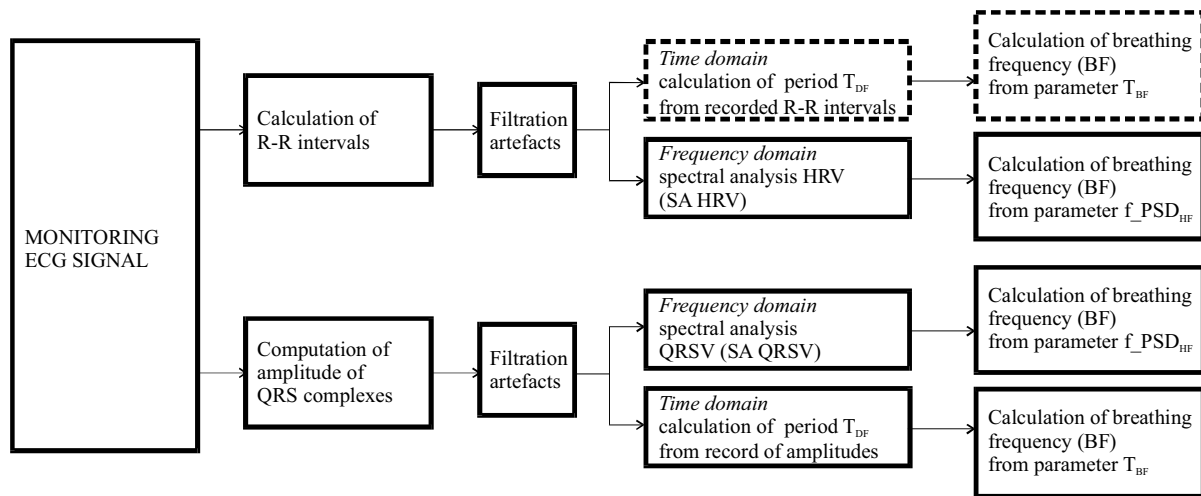
Fig. 2 Summary of methods allowing assessment of breathing frequency from ECG signal
