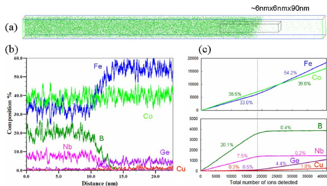
FIG. 3. (a) 3DAP elemental map and [(b) and (c)] concentration depth profiles obtained from a selected volume of 6 \times 6 \times 90\text{ nm}^3 .
