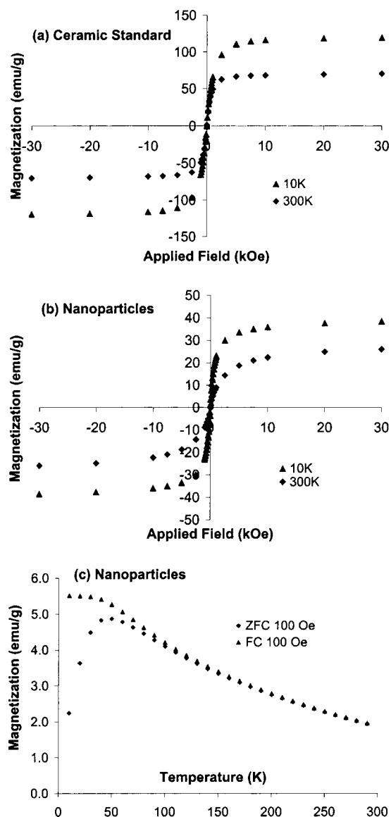
FIG. 3. (a) Hysteresis loop for NZFO bulk ceramic standard (b) and NZFO nanoparticles, measured at ( \blacktriangle ) 10 K and ( \blacklozenge ) 300 K. (c) Magnetization vs temperature plot for the nanoparticles.
