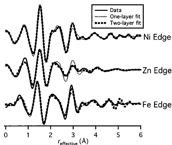
FIG. 4. Real part of the EXAFS Fourier transforms for the three metallic constituents. Fits using the one-layer and two-layer models are also shown.
