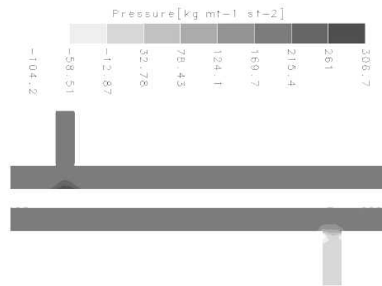
Figure 8 | Pressure contours on a centrally located xz plane for configuration 1.
