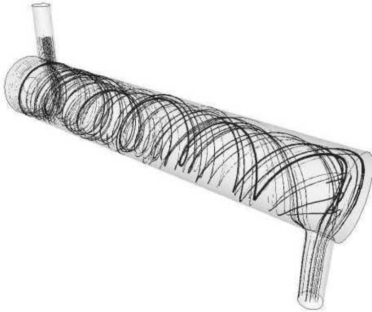
Figure 11 | Particle tracks coloured by dose for configuration 3.
