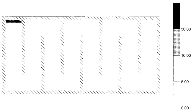
Figure 8 | DCAA concentration (in \mu\text{g l}^{-1} \times 10,000 ) after simulation time of 0.07 min.
