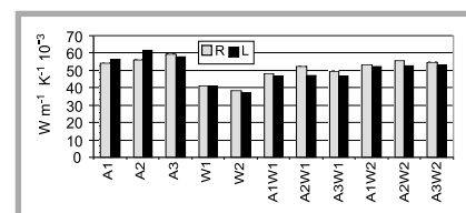
Figure 2. The thermal conductivity of the textile materials.
