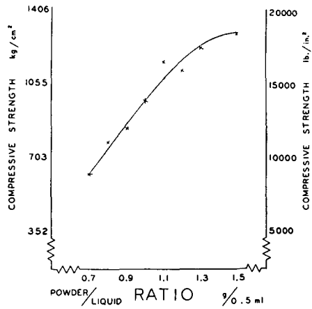
Fig. 2 Mean compressive strength values for mixes of different powder/liquid ratios.
