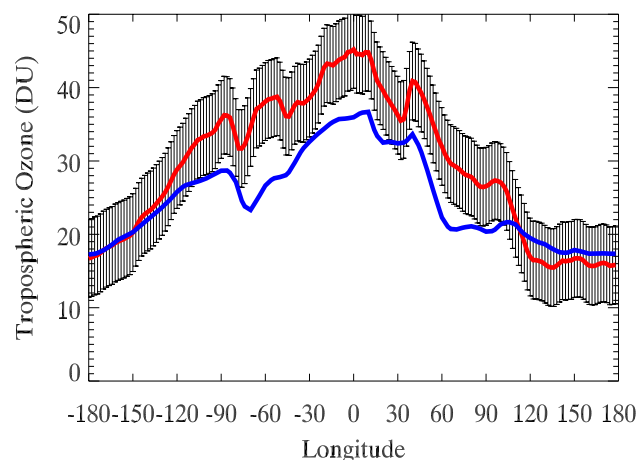
Fig. 2. The meridionally averaged zonal TTOC distribution in model calculated (blue) and satellite retrieved (red) TTOC for September 1992. This distribution is used to define a measure of error according to Eq. (1). The shaded lines denote one-sigma standard deviation (5.3 DU). Atlantic ozonesonde and aircraft ozone data (taken within longitudes 35W to 15E) during September and October 1992 fall within the shaded region.
