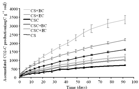
Fig. 1: Accumulated average CO 2 -C production (mg C g -1 soil) with incubation time. Vertical lines show the standard errors of the means
