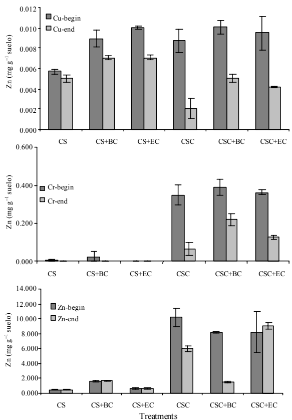
Fig. 2: Trace elements concentration in different treatments from the beginning (i) to the end (f) of the incubation test. Trace elements of treatments CS, CS+BC and CS+CE were multiplicity for 10. Vertical lines represent the standard errors of the means
