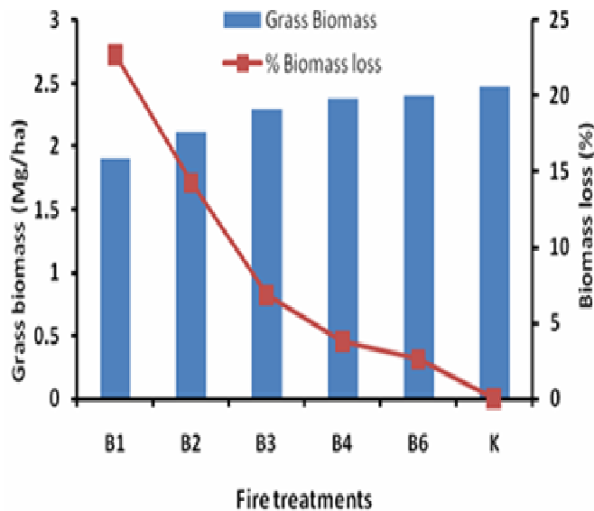
Figure 1. Effects of long term fire treatment on change in grass biomass production over 26 years. B1= annual burning, B2 = biennial burning, B3 = triennial burning, B4= Quadrennial, B6 = Sexennial, K = Control
