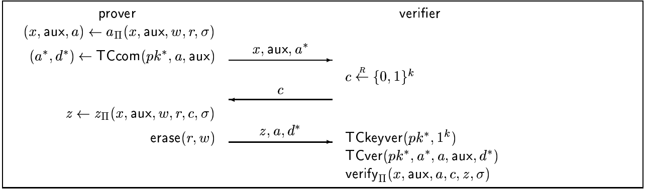
Figure 5: \text{UC}_{[pk^*, \sigma]}^R(x; \text{aux}) : A UCZK protocol for R with common reference string (pk^*, \sigma) drawn from \mathcal{D}_{pk}(\text{TC}) \times \mathcal{D}_{\sigma}(\Omega^R) , common input x , and auxiliary input \text{aux} where \Pi = \Omega_{\sigma}^R(x; \text{aux}) .
