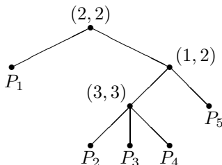
FIG. 2 Labeled tree for an iterated access structure.
