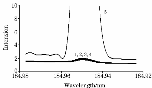
Fig. 9 Na to Hg spectral interaction line
