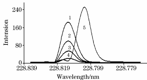
Fig. 8 As to Cd Spectral Interaction line
