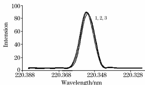
Fig. 4 Sample flow influence for Pb
