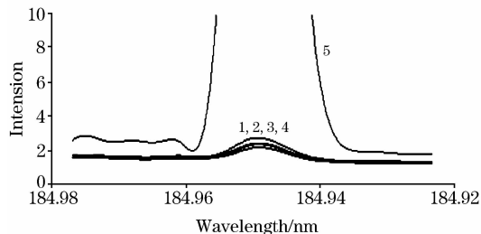
Fig. 10 Sn to Hg spectral interaction line
