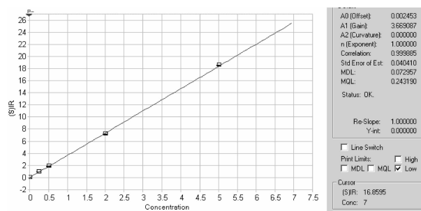
Fig. 5 Pb stand curve
