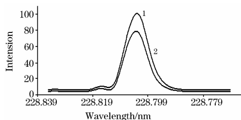
Fig. 2 Nebulizer pressure influence for Cd
