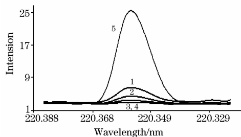
Fig. 7 Cu to Pb spectral interaction line
