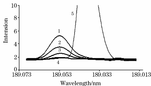
Fig. 6 Cr to As spectral interaction line
