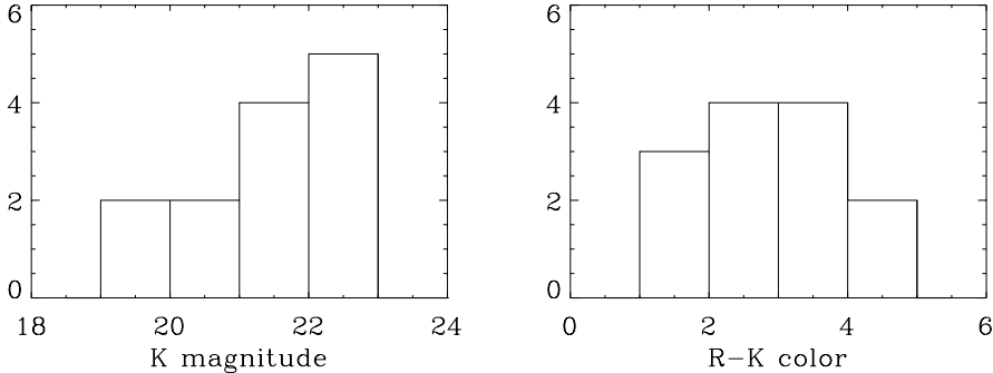
Figure 1. Left: K magnitude histogram of GRB host galaxies. Data were obtained as part of our on-going K -band imaging program on the VLT for 40%, the other photometric data points are quoted from Fruchter et al. (1999), Djorgovski et al. (2000), Vreeswijk et al. (1999), Bloom et al. (1999), Klose et al. (2000), Chary et al. (2002). Right: histogram of the observed R-K colors, for the similar sample of GRB hosts. The R magnitudes were taken from the literature, see Djorgovski et al. 2001 for references.
