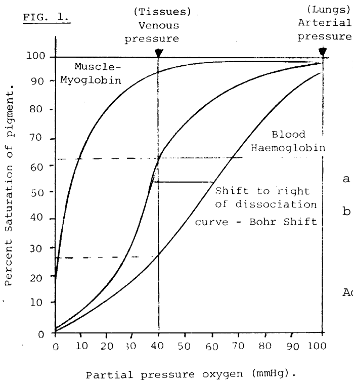
FIGURE I OXYGEN DISSOCIATION CURVES FOR MAMMALIAN MYOGLOBIN AND HAEMOGLOBIN AT BODY TEMPERATURE
