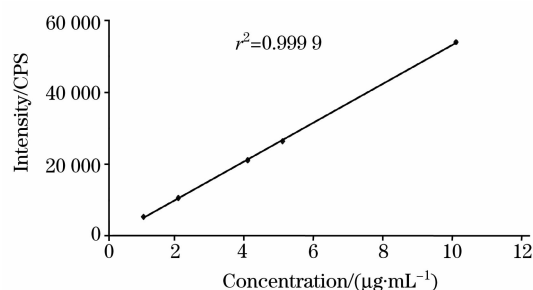
Fig. 2 Arsenic linear fitted calibration curve
