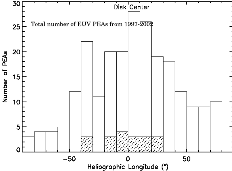
Figure 5. Distribution of PEAs in heliographic longitude in bins of 10 degrees as identified in EIT 195 Å images from 1997–2002. The portions of the bars presented as the spotted areas represent those PEAs for which no white-light CME had been detected by LASCO/C2 (adopted from Tripathi et al. (2004)).
