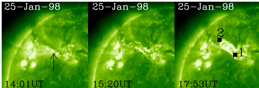
Figure 1. Images taken by EIT at 195 \text{ \AA} on 25 January 1998. The first two images show the eruption of a prominence (marked with an arrow in the left panel) and the consequent post-eruptive arcade. The right panel shows the post-eruptive arcade at times of its maximum evolution (emission). Point ‘1’ and ‘2’ represent the two extreme end-points of the post-eruptive arcade. In the images north points upwards and west towards the right.
