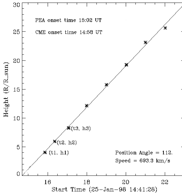
Figure 4. Height-time diagram for the leading edge of the CME observed on 25 January 1998 as provided by LASCO/C2 and C3 observations. h1 is the height measured at time t1, h2 is measured at t2 and so on. Approximate timings of CME (triangle) and PEA (solid dot) onset is marked in the figure.
