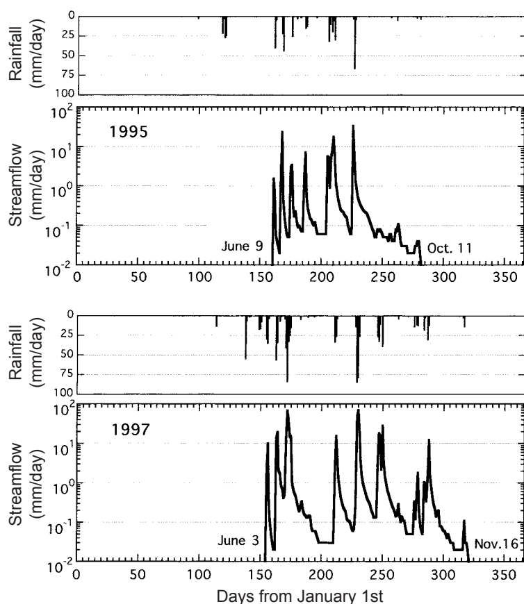
Fig. 2. Typical annual hydrographs at the catchment
