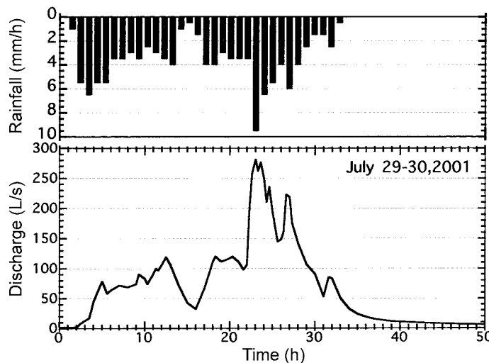
Fig. 3. Typical storm hydrograph at the catchment
