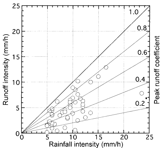
Fig. 6. Peak runoff coefficient
