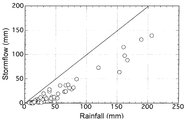
Fig. 5. Relationship between rainfall and stormflow
