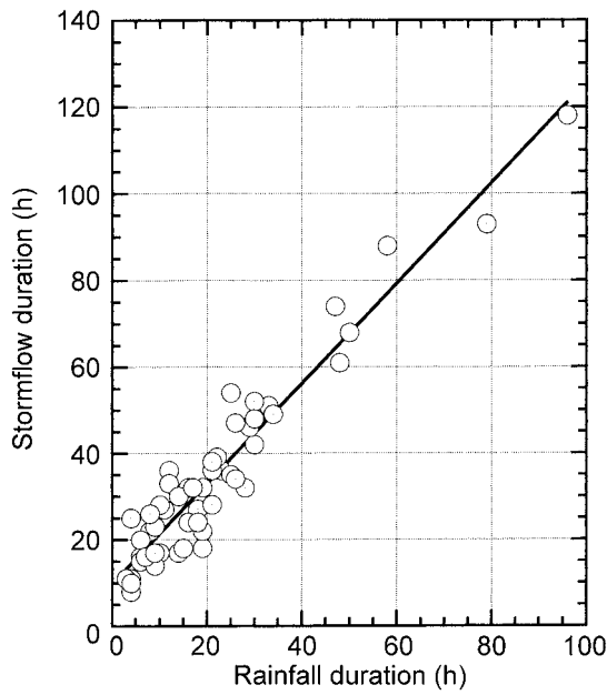
Fig. 4. Relationship between rainfall duration and storm duration
