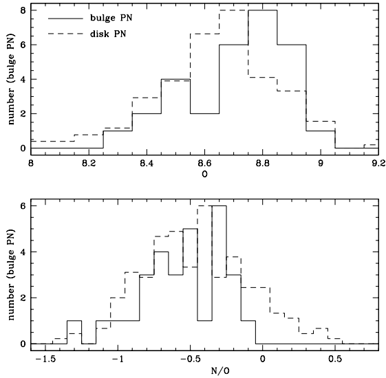
Fig. 1. Top panel: Oxygen abundance distribution, on a logarithmic scale, where 12 is the abundance of hydrogen. Bottom panel: Nitrogen over oxygen ratio distribution.
