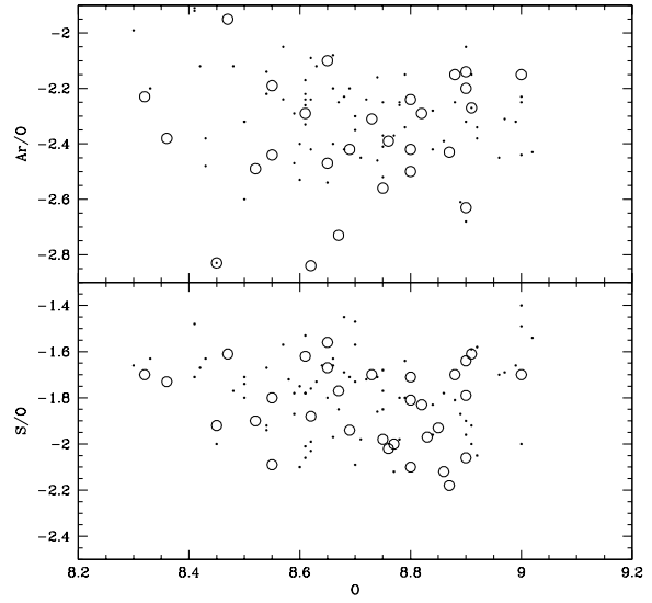
Fig. 2. Ar/O and S/O ratios as a function of the oxygen abundance. Dots represent bulge PNe, points Type II PNe of the disk.
