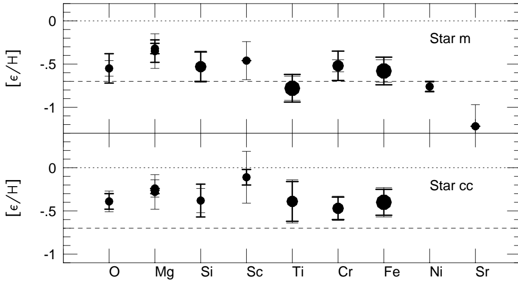
Fig. 1. Elemental abundances for Star ‘m’ (top) and Star ‘cc’ (bottom) relative to the the Sun. Two errorbars are shown for each point; thick line for the line-to-line scatter, and thin line for the systematic uncertainties in the model atmospheres analysis. The largest data points include \geq 16 line abundances, and the smallest include \leq 5 . The mean SMC underabundance is noted by the dashed line (although note that the SMC A-supergiant Sr result is off the dashed line and this graph at -1.7 ).
