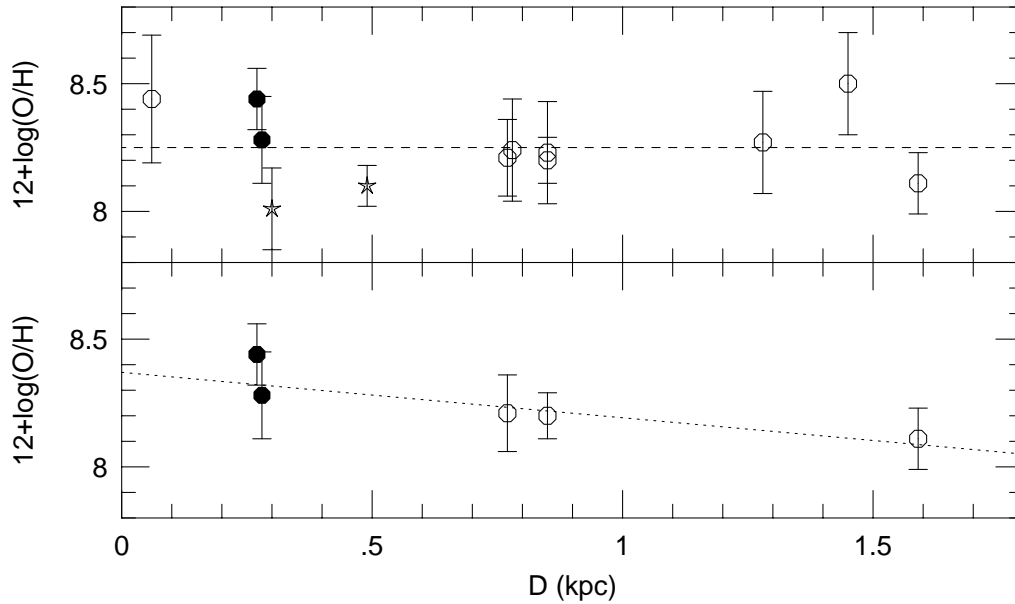
Fig. 2. Oxygen abundances versus NGC 6822 galactocentric distance. Filled circles represent the stellar data, hollow circles show the Pagel et al. (1980) nebular data, and asterisks note two planetary nebulae results from Richer & McCall (1995). The dashed line in the top panel shows the mean oxygen abundance from Pagel et al. ( 12 + \log(\text{O}/\text{H}) = 8.25 ). In the bottom panel, only the stellar abundances and those from H II regions where O III was detected are shown. A least squares fit to the data ( dotted line ) suggests a slope of -0.18 dex/kpc.
