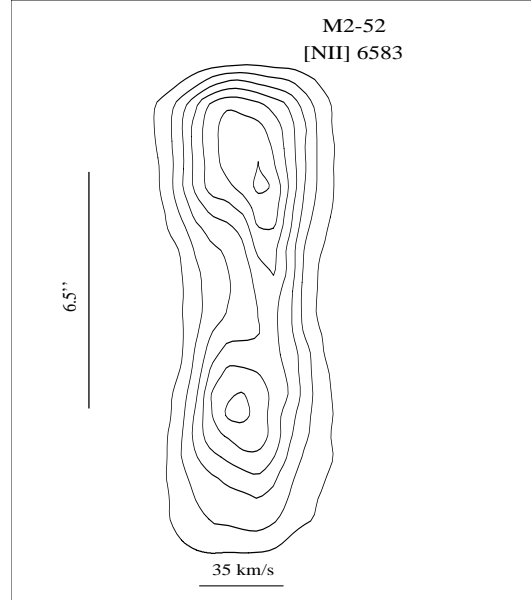
Fig. 1. Contour diagram of the [N II] 6583 emission line in the bi-dimensional spectrum. The spatial direction is along the y axis. The two knots detected are oriented E-W (East is up), and separated by 6.5'' . The stellar continuum should be located between the knots, but the star is too faint to be detected in our echelle spectrum. The emission is filling the slit of 13.3'' length. The FWHM of the [N II] line is 0.95 \text{ \AA} , equivalent to a velocity range of 35 \text{ km s}^{-1} .
