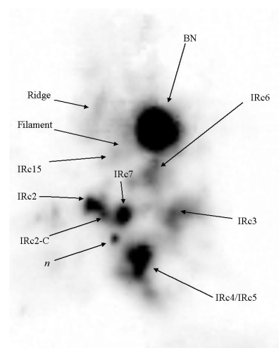
Fig. 1. 10 \mu\text{m} image of the BN/KL nebula. North is up, East to the left.
