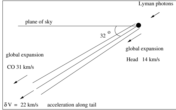
Fig. 3. A schematic model of the Helix cometary Knot 38 which has the longest tail. This tail is tilted at 32 degrees away from the observer and is accelerating along its length. The global expansion of the system of Helix cometary knots is measured as 14 \text{ km s}^{-1} .
