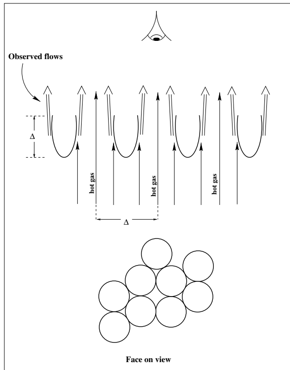
Fig. 9. A sketch of a model of the Honeycomb nebula. The morphology is generated as a supernova blast wave breaks through the weak points of an unstable old giant shell. The weak points are separated by approximately the thickness of the old shell.
