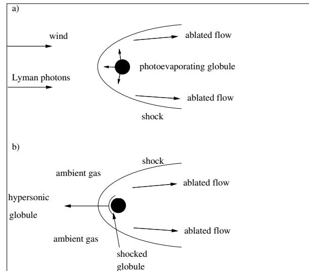
Fig. 1. Two possibilities for the creation of ablated flows are illustrated. (a) A particle wind causes an ablated flow from a globule with a photoionized surface. (b) Shocked ambient gas mixes with evaporating material from the surface of a globule traveling at hypersonic speeds.
