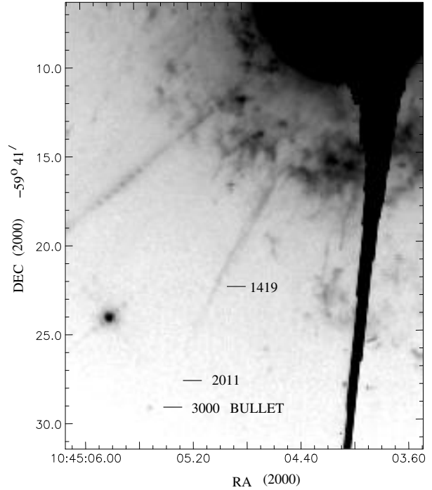
Fig. 4. An HST image where Finger 1 is seen projecting from Eta Carinae. The measured outflowing speeds are shown in \text{km s}^{-1} at two positions along its length as is that of the “bullet” at its tip. Deceleration towards Eta Carinae could be indicated. The other spikes are diffraction artefacts.
