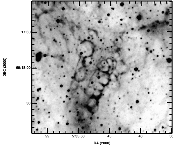
Fig. 8. An image of the Honeycomb nebula in the halo of 30 Doradus.
