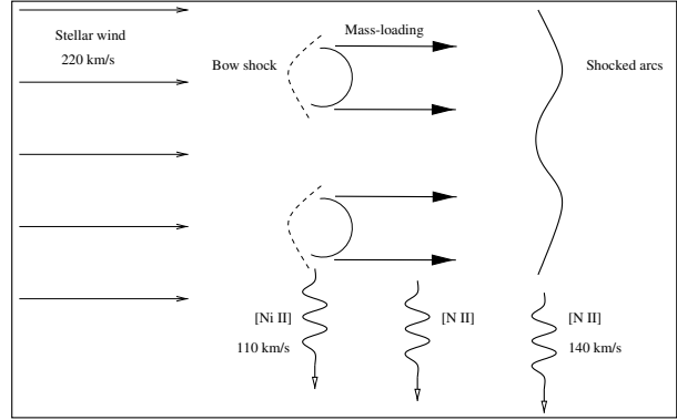
Fig. 7. A model invoking ablated flows to explain the difference in expansion velocities of the shell of [\text{Ni II}] \lambda 7412 \text{ \AA} emitting globules and the [\text{N II}] \lambda 6584 \text{ \AA} emitting envelope of the inner shell of P Cygni is shown.
