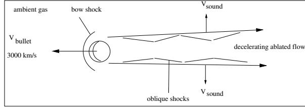
Fig. 5. A model of Finger 1 invoking ablated flows is shown. The finger will have a high aspect ratio for it expands perpendicularly only at the sound speed ( \approx 10 \text{ km s}^{-1} ) and will be decelerated towards Eta Carinae by the “friction” of oblique shocks.
