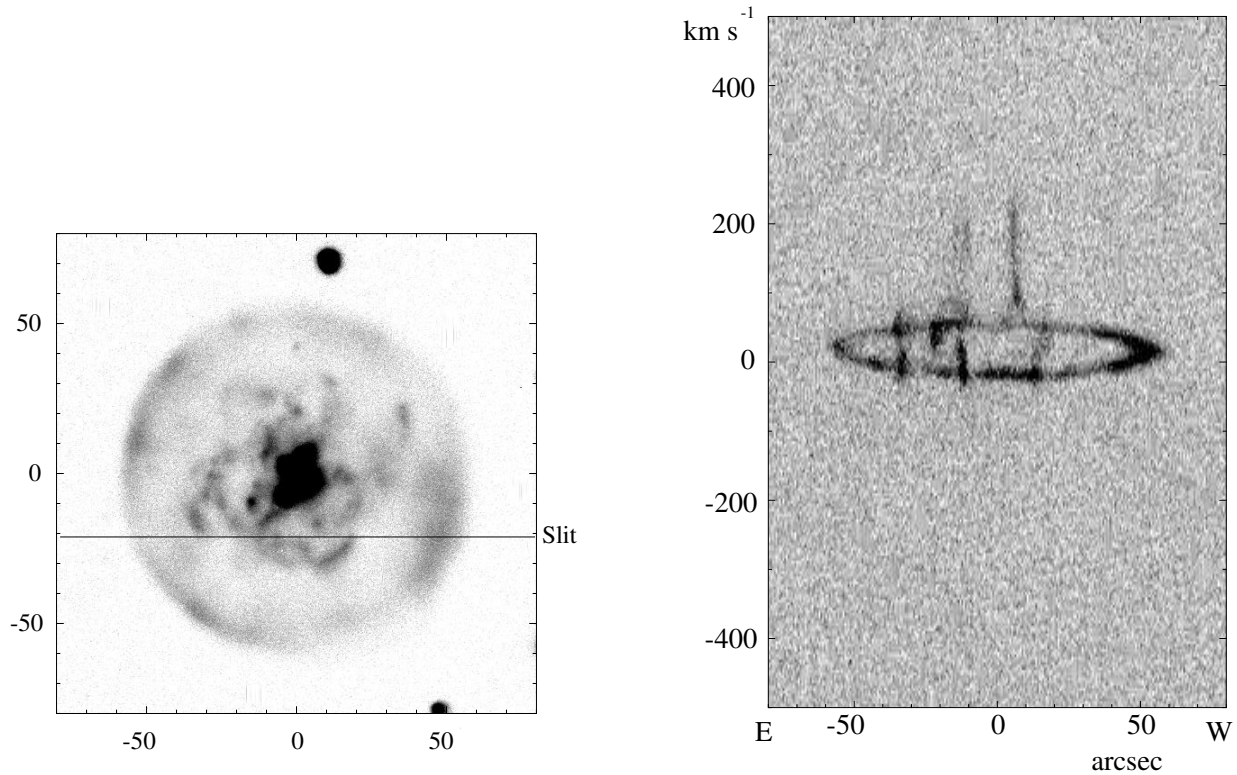
Fig. 2. A slit position is shown across an [O III] 5007 Å image (left panel) of Abell 30. The pv array (right panel) shows both the radial expansion of the hydrogen rich outer shell and velocity spikes over the inner hydrogen-deficient outflows. The radial velocity scale is heliocentric.
