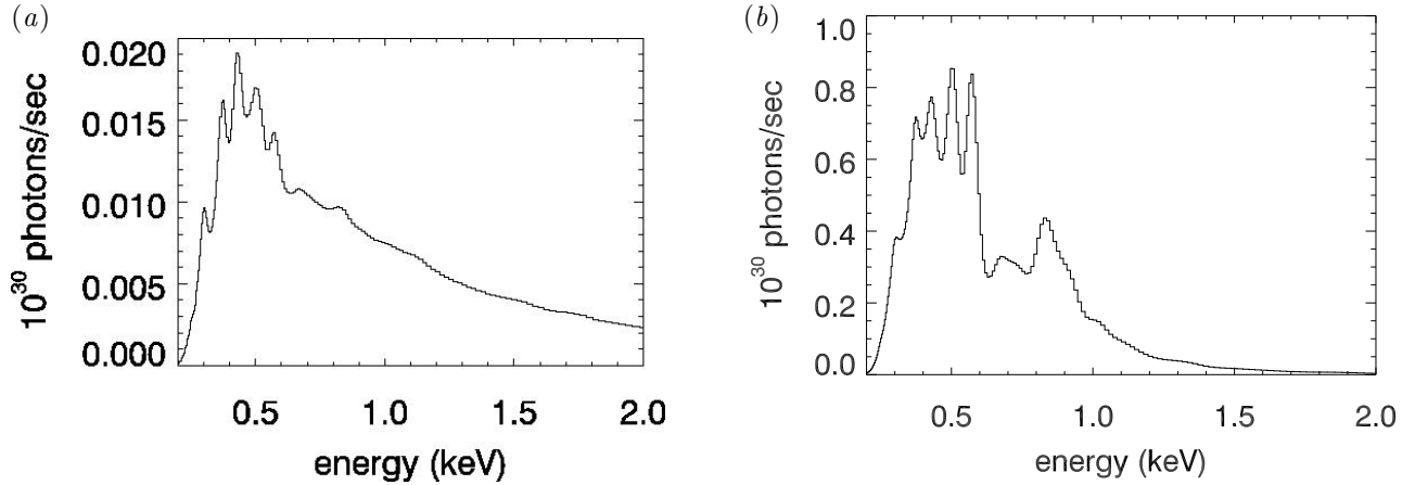
Fig. 1. Synthesized X-ray spectra calculated from the density, temperature and abundance distribution of a simulation of two interacting winds: (a) without thermal conduction; (b) with 1% efficient thermal conduction. The parameters of the winds were: \dot{M}_{\text{AGB}} = 2 \times 10^{-5} M_{\odot} \text{ yr}^{-1} , v_{\text{AGB}} = 10 \text{ km s}^{-1} , \dot{M}_{\text{fast}} = 10^{-7} M_{\odot} \text{ yr}^{-1} , v_{\text{fast}} = 2000 \text{ km s}^{-1} . The H I column density between us and the PN is taken to be 9 \times 10^{20} \text{ cm}^{-2} . The spectra are smoothed to approximate the resolution of the Chandra ACIS spectral resolution, but were not convolved with the instrumental response function.
