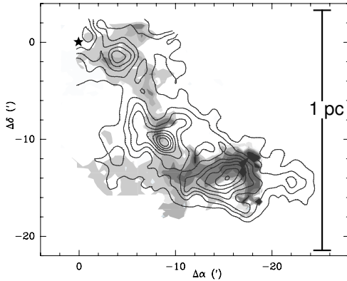
Fig. 1. ^{12}\text{CO}(1-0) integrated intensity map of the HH 300 redshifted molecular outflow lobe, superimposed on a grayscale map of the ^{13}\text{CO} line width (FWHM). Darker tones show regions of wider ^{13}\text{CO} spectra. Coordinate offsets are given with respect to the outflow source position (star symbol). From Arce & Goodman (2001).
